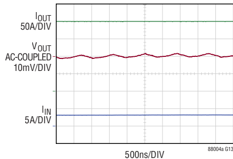
FIGURE 10 CIRCUIT V_{IN} = 54V , V_{OUT} = 0.75V , f_{SW} = 550kHz 200A LOAD ON V_{OUT}
