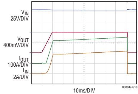
54V IN OCP
