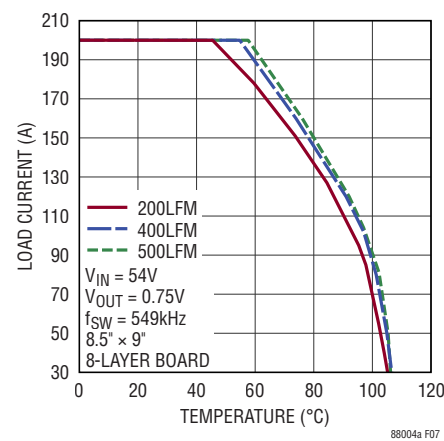
Figure 7. Thermal Derating 48VIN, 0.75VOUT
