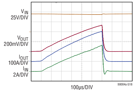
45V IN Short-Circuit Start-Up
