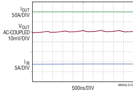
FIGURE 10 CIRCUIT V_{IN} = 45V , V_{OUT} = 0.75V , f_{SW} = 550kHz 200A LOAD ON V_{OUT}
