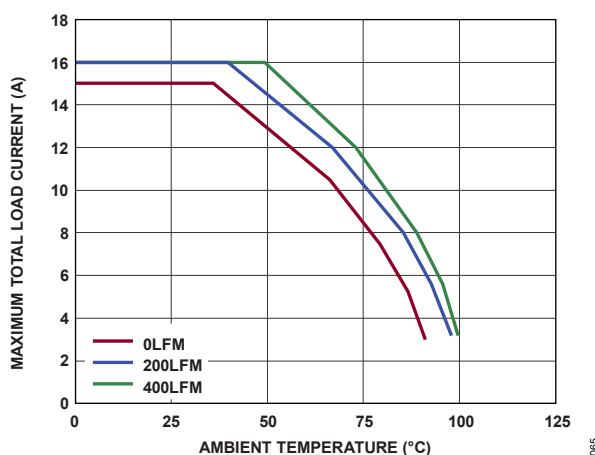
Figure 65. 36V IN to 5V OUT Derating with Airflow
