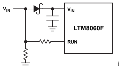
Figure 66. The Input Diode Prevents a Shorted Input from Discharging a Backup Battery Connected to the Output. It also Protects the Circuit from a Reversed Input, the LTM8060F Runs only when the Input is Present
