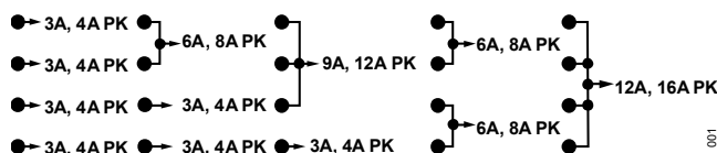
Figure 1. Configurable Output Array
