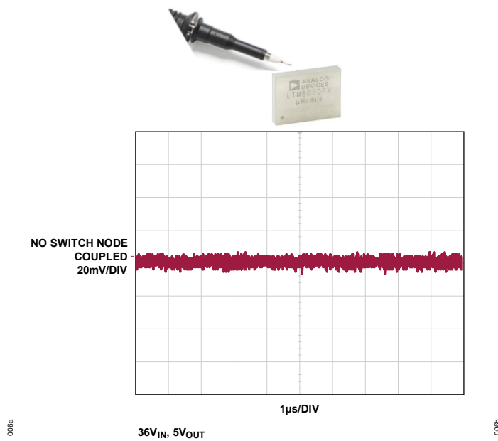
(b) LTM8060F with EMI Shielding
