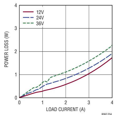
Figure 4. Power Loss Curves, 5V OUT Still Air
