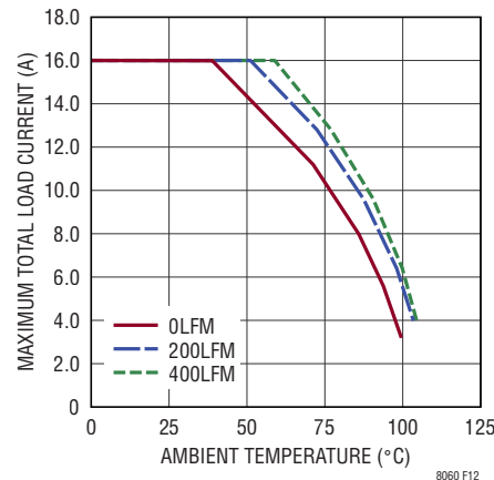
Figure 12. 24V IN to 5V OUT Derating with Airflow
