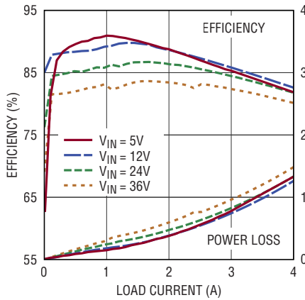
Efficiency and Power Loss V_{OUT} = 1.5\text{V} , BIAS = 5V, Burst Mode
