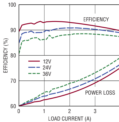
Efficiency and Power Loss V_{OUT} = 3.3\text{V} , BIAS = 5V, Burst Mode
