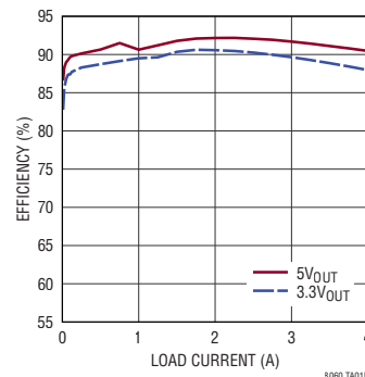
Efficiency, V_{IN} = 24\text{V} , BIAS = 5V
