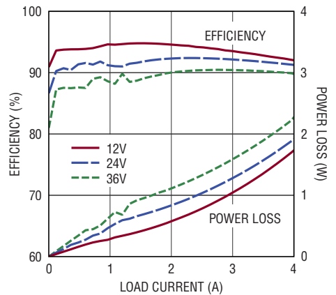
Efficiency and Power Loss V_{OUT} = 5\text{V} , BIAS = 5V, Burst Mode
