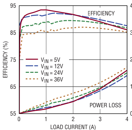
Efficiency and Power Loss V_{OUT} = 2.5\text{V} , BIAS = 5V, Burst Mode
