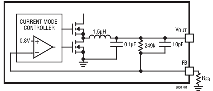
Figure 1. Set Output Voltage with a FB Resistor
