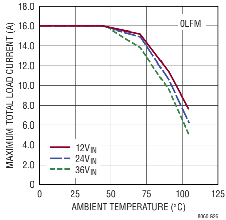
Derating, V_{OUT} = 2V BIAS = 5V, DC2820A Demo Board T_J = 120^\circ\text{C} , Burst Mode All Channels at Same Load
