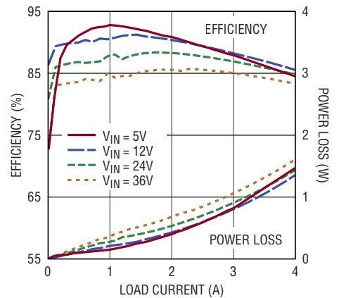
Efficiency and Power Loss V_{OUT} = 2\text{V} , BIAS = 5V, Burst Mode
