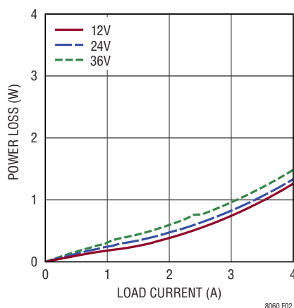
Figure 2. Power Loss Curves, 1.5V OUT Still Air
