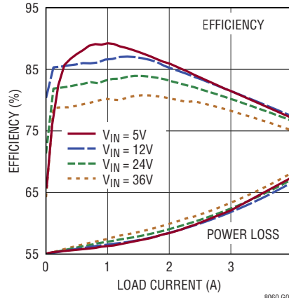
Efficiency and Power Loss V_{OUT} = 1\text{V} , BIAS = 5V, Burst Mode
