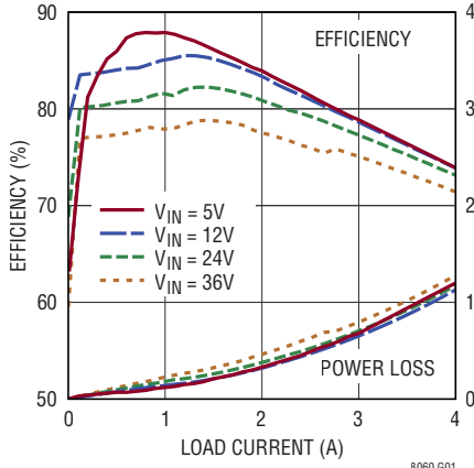
Efficiency and Power Loss V_{OUT} = 0.8\text{V} , BIAS = 5V, Burst Mode
