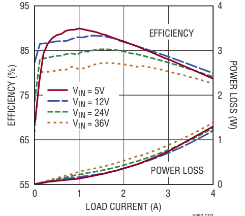
Efficiency and Power Loss V_{OUT} = 1.2\text{V} , BIAS = 5V, Burst Mode
