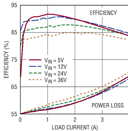
Efficiency and Power Loss V_{OUT} = 1.8\text{V} , BIAS = 5V, Burst Mode
