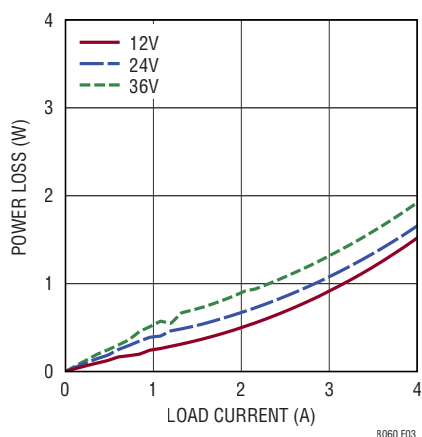
Figure 3. Power Loss Curves, 3.3V OUT Still Air
