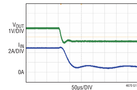
Short-Circuit with 10A Load
