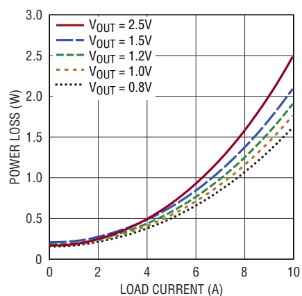
Figure 7. Power Loss vs Load Current at 3.3VIN
