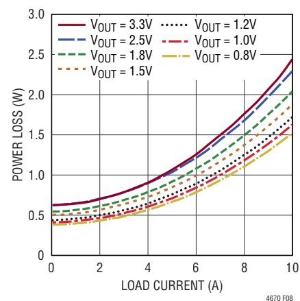
Figure 8. Power Loss vs Load Current at 5.5VIN
