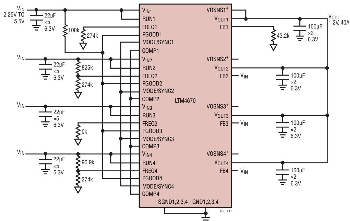
Figure 17. Four-Phase, 2MHz, 1.2V, 40A Design
