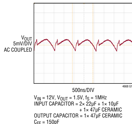
Output Ripple
