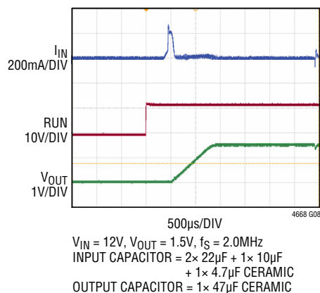
Start-Up with No Load
