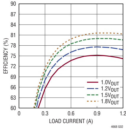
Efficiency vs Load Current at 12V IN
