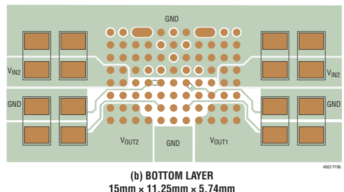
Figure 19. Recommended PCB Layout
