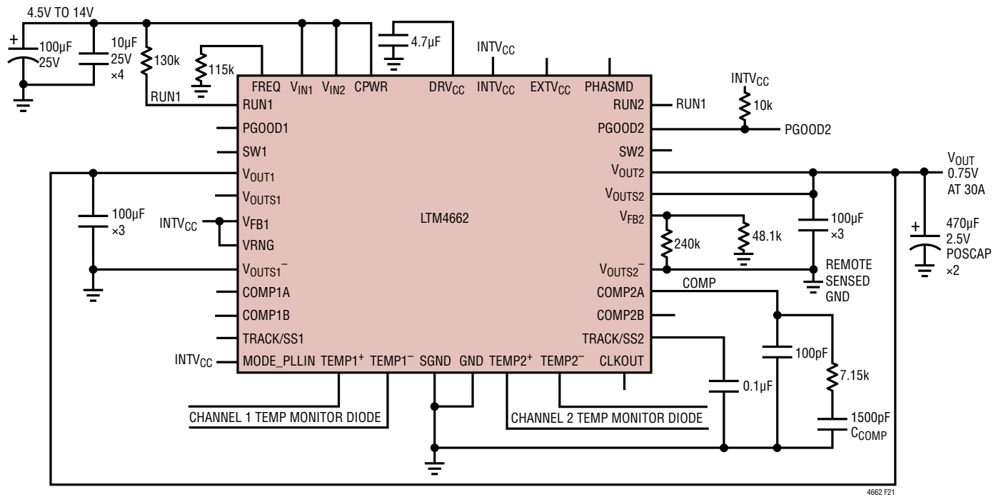
Figure 21. 12V Input to 0.75V at 30A 2-Phase
