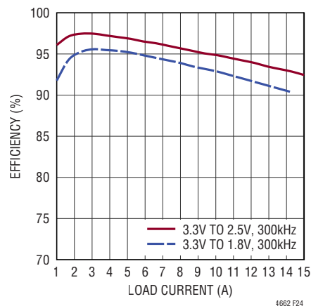
Figure 24. Efficiency, 3.3VIN
