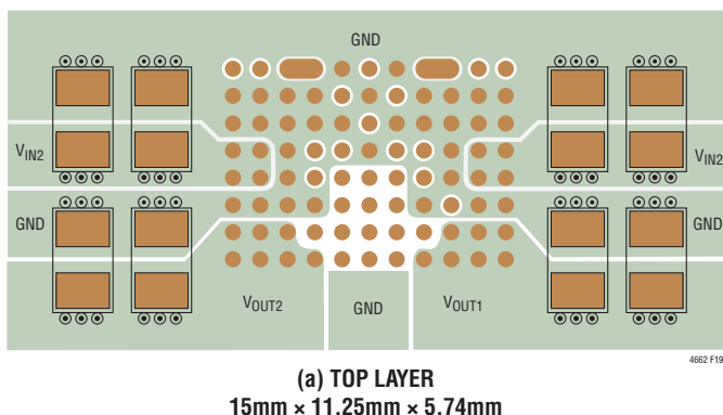
Figure 19. Recommended PCB Layout
