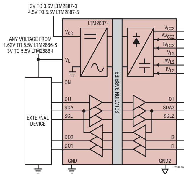
Figure 4. V_{CC} and V_L Are Independent
