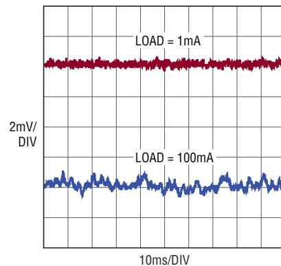
V_{CC2} or V_{L2} Noise
