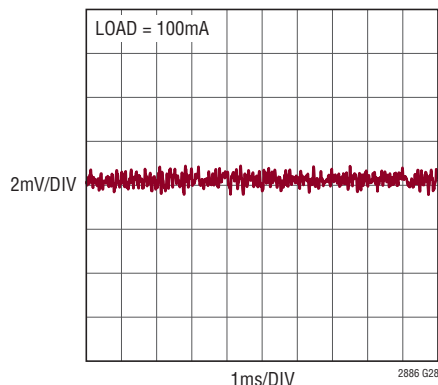
V_{CC2} Noise
