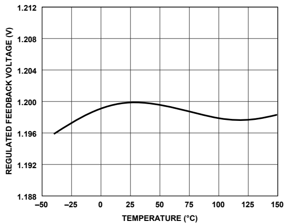
Figure 12. Regulated Feedback Voltage vs. Temperature
