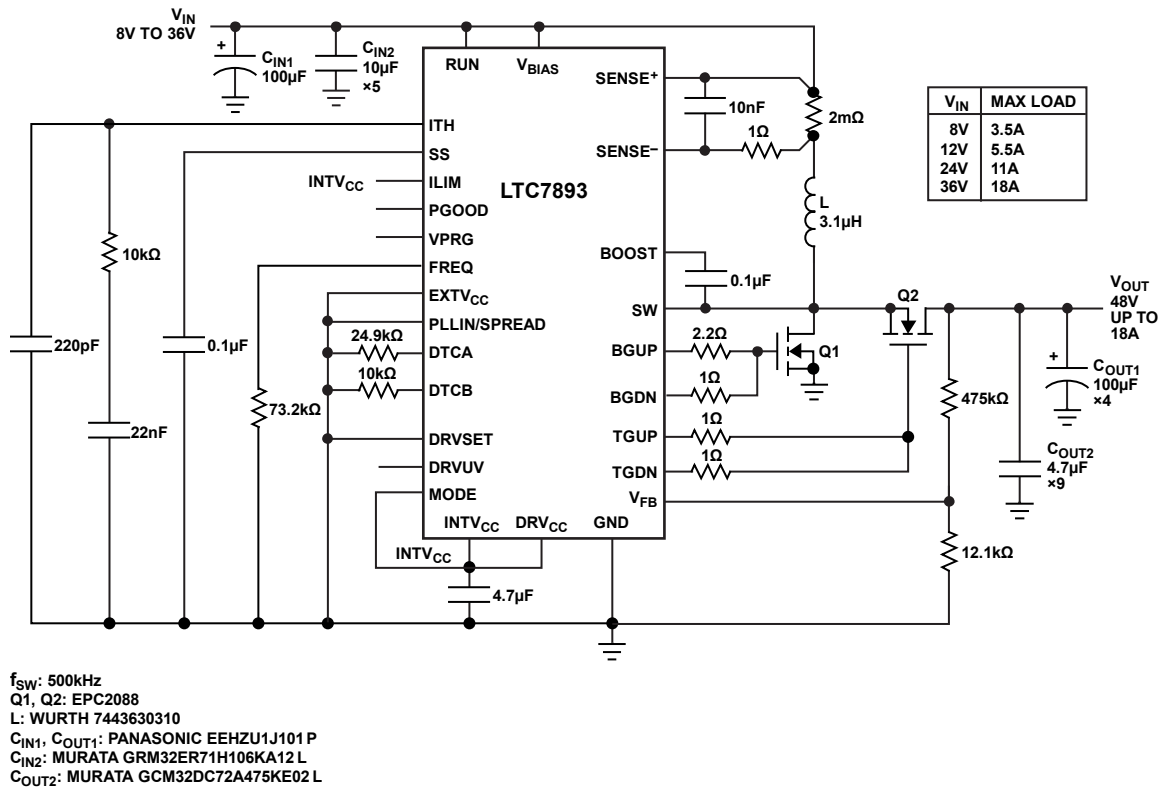
Figure 54. High Efficiency, 48V OUT , Boost Regulator Using GaN FETs
