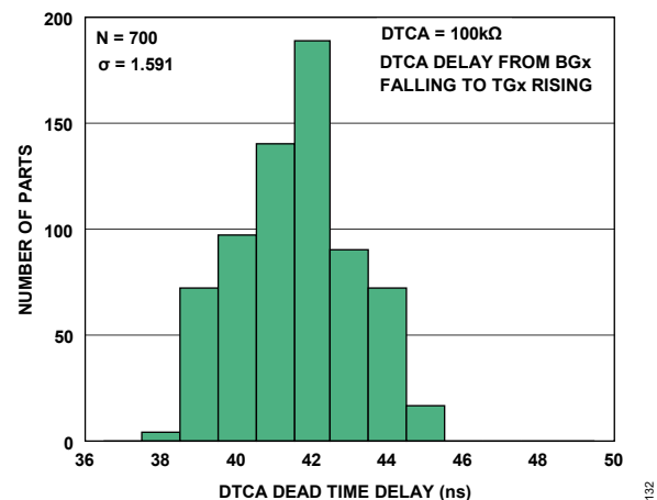
Figure 32. DTCA = 100kΩ Dead Time Delay Histogram
