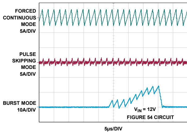
Figure 10. Inductor Current at Light Load
