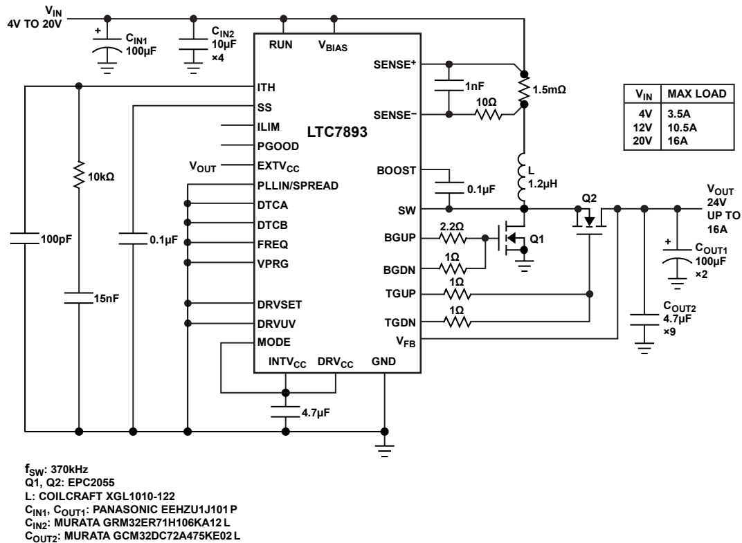
Figure 48. High Efficiency, 24V OUT , Boost Regulator Using GaN FETs
