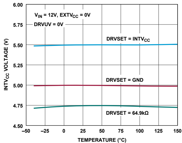
Figure 26. INTV_{CC} Voltage vs. Temperature
