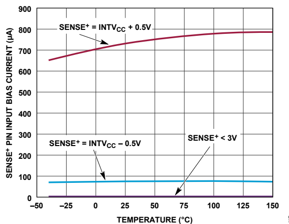
Figure 17. SENSE+ Pin Input Current vs. Temperature
