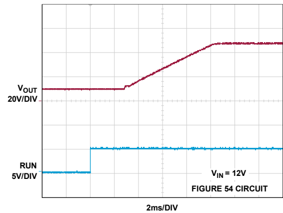
Figure 11. Soft Start-Up
