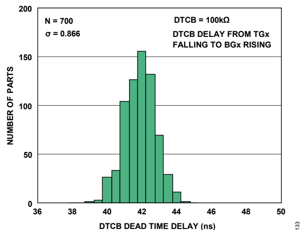
Figure 33. DTCB = 100kΩ Dead Time Delay Histogram
