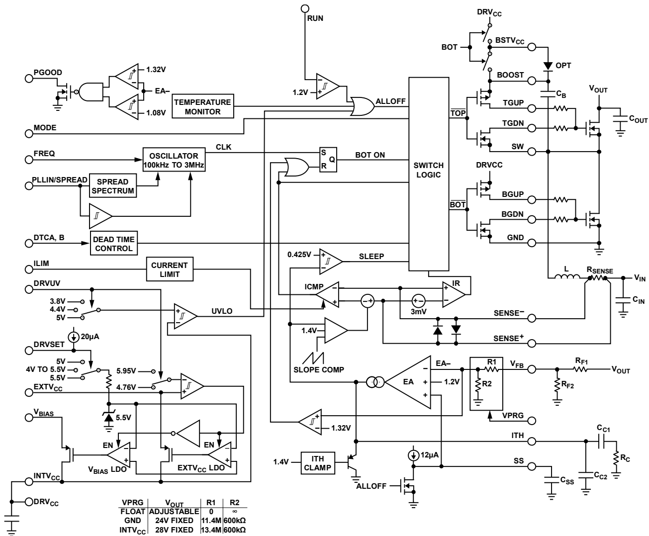
Figure 34. Functional Diagram
