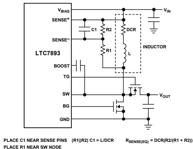
Figure 37. Using the Inductor DCR to Sense Current ( R_{\text{SENSE(EQ)}} is the Equivalent Sensed Resistance)
