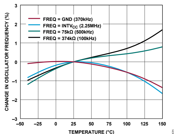
Figure 21. Oscillator Frequency vs. Temperature
