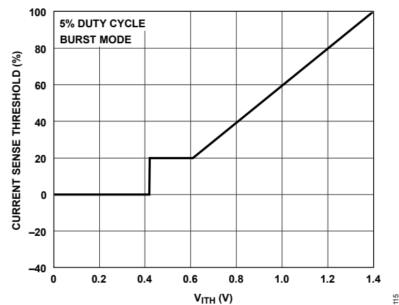
Figure 15. Maximum Current Sense Threshold Relative to V_{SENSE(MAX)} vs. V_{ITH} in Burst Mode
