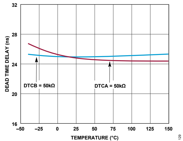
Figure 29. Dead Time Delay vs. Temperature
