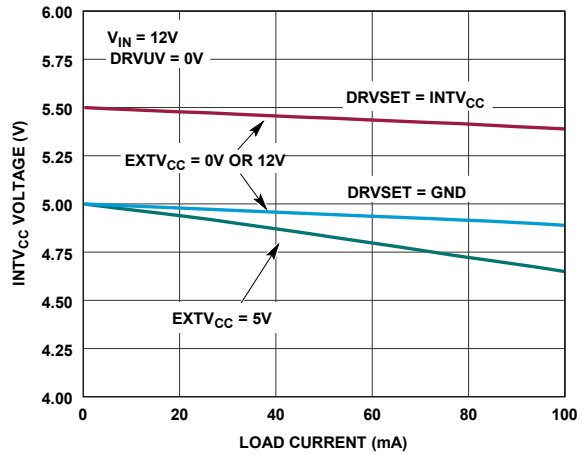
Figure 24. INTV_{CC} Voltage vs. Load Current
