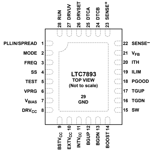
Figure 3. Pin Configuration
