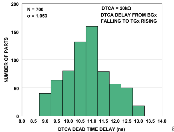
Figure 30. DTCA = 20kΩ Dead Time Delay Histogram
