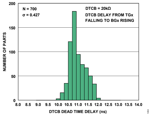
Figure 31. DTCB = 20kΩ Dead Time Delay Histogram
