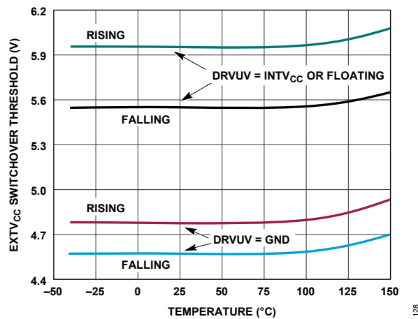
Figure 28. EXTV CC Switchover Threshold vs. Temperature
