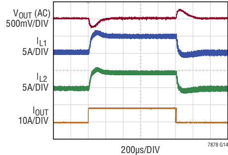
Two-Phase Parallel Operation Load Step ( 12V_{IN} , 12V_{OUT} )
