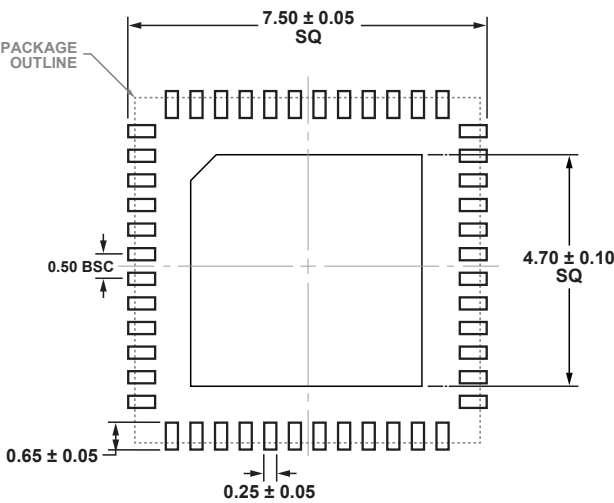
RECOMMENDED SOLDER PAD LAYOUT (TOP VIEW)
