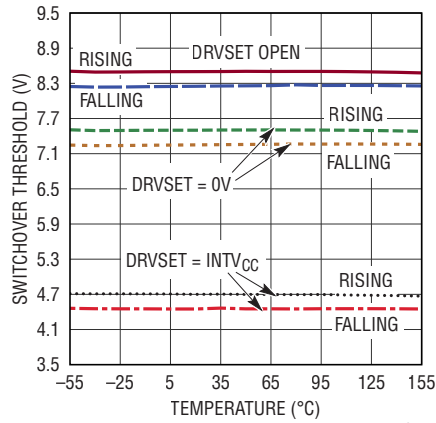
EXT CC Switchover Thresholds vs Temperature
