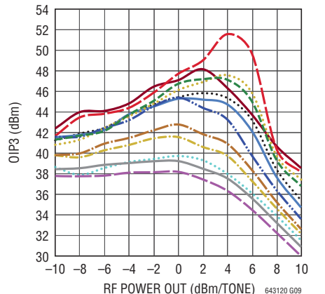
OIP3 vs Power Out Over Frequency
