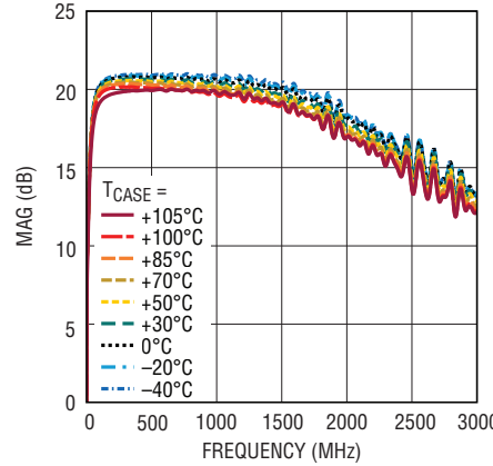
S21 vs Frequency Over Temperature
