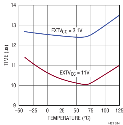
GATE Break-Before-Make Time vs Temperature
