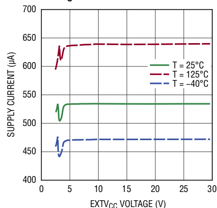
Total Supply Current vs EXTV CC Voltage
