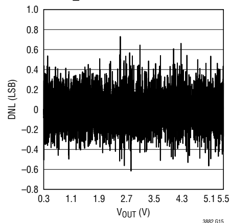
V_{OUT\_COMMAND} DNL
