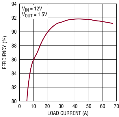
Efficiency vs Load Current (3-Phase Using D12S1R845A Power Block)
