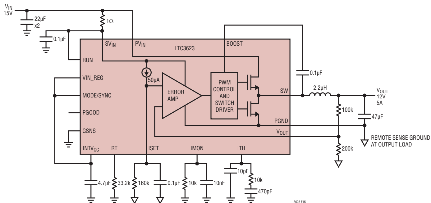
Figure 15. 15V to 12V 1MHz Buck Converter with Output Resistor Dividers
