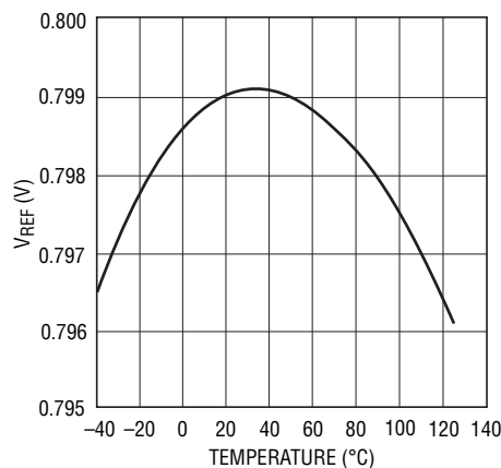
V_{REF} vs Temperature, V_{IN} = 3.3V
