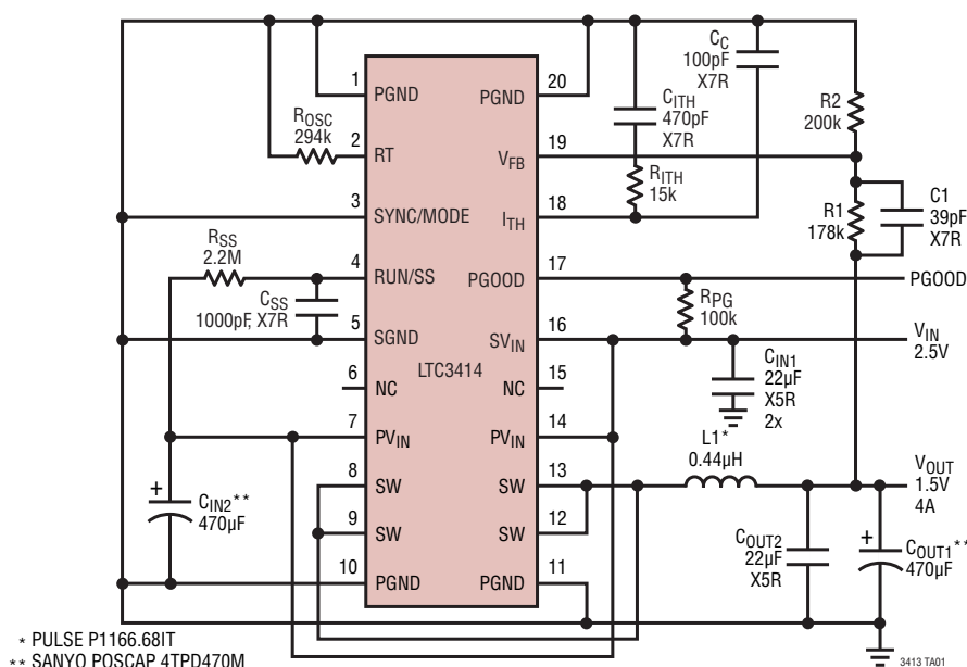
1.5V, 4A Step-Down Regulator at 1MHz, Burst Mode
