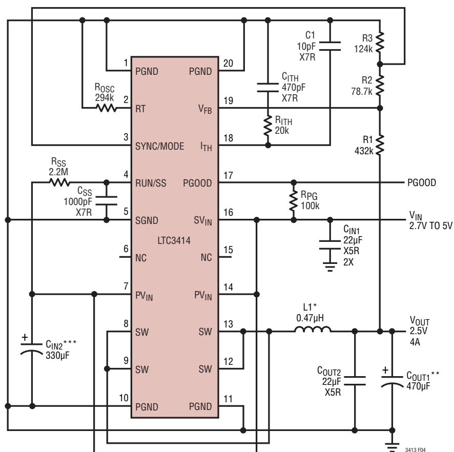
Figure 4. 2.5V, 4A Regulator at 1MHz, Burst Mode Operation
