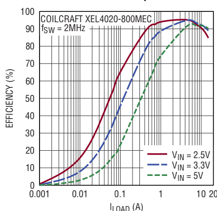
Efficiency, V_{OUT} = 1.8V Forced Continuous Operation
