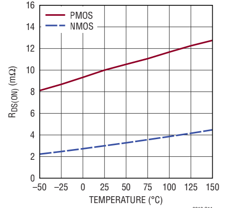
Switch-On Resistance
