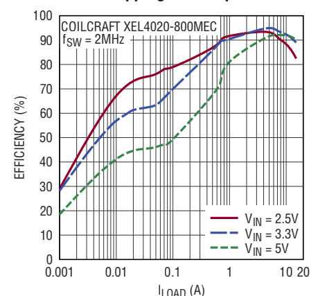
Efficiency, V_{OUT} = 1.8V Pulse-Skipping Mode Operation
