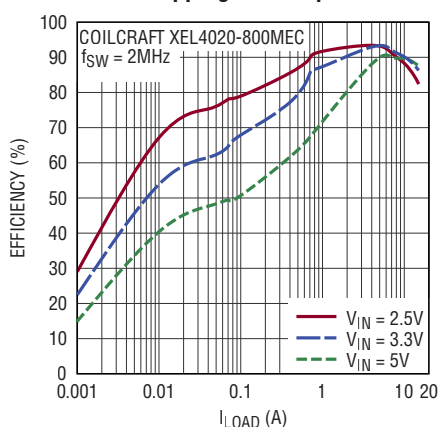
Efficiency, V_{OUT} = 1.2V Pulse-Skipping Mode Operation
