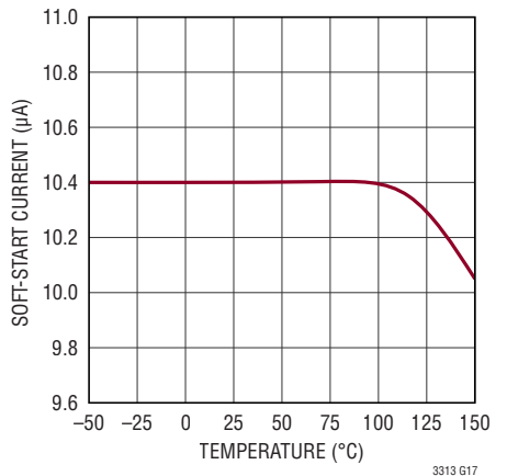
Soft-Start Current
