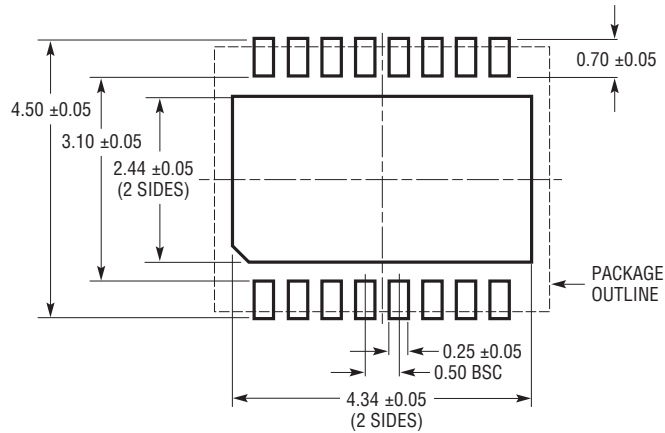
DHD Package 16-Lead Plastic DFN (5mm × 4mm) (Reference LTC DWG # 05-08-1707 Rev A)
