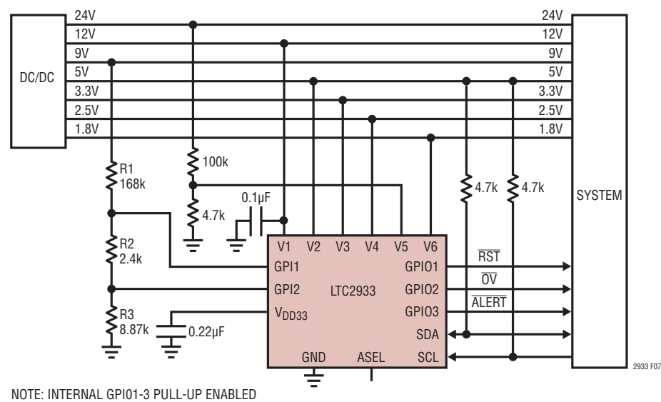
Figure 7. 7-Power Supply Monitor
