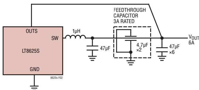
Figure 2. Additional Output Ripple Filtering Using Feedthrough Capacitors
