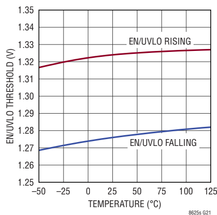
EN/UVLO Pin Thresholds
