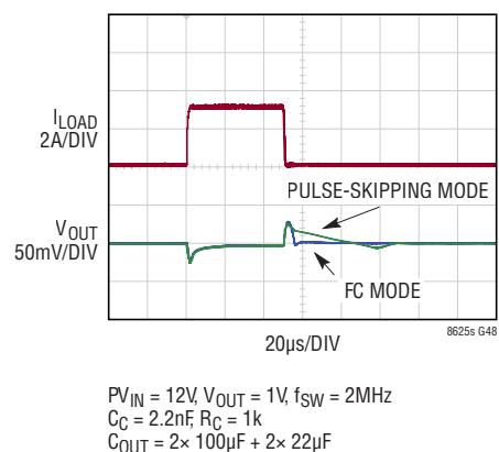
Transient Response: Load Current Stepped from 100mA to 3.1A
