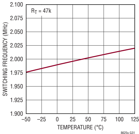
Switching Frequency
