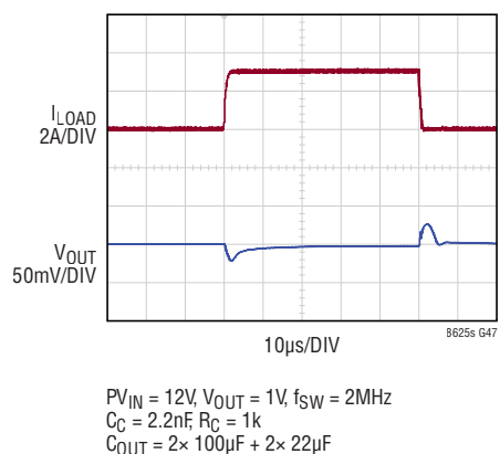
Transient Response: Load Current Stepped from 2A to 5A
