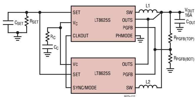
Figure 12. Paralleling Two LT8625S Devices
