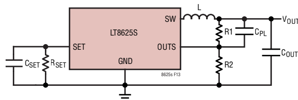
Figure 13. Configuring the LT8625S for Output Voltages Above 6V
