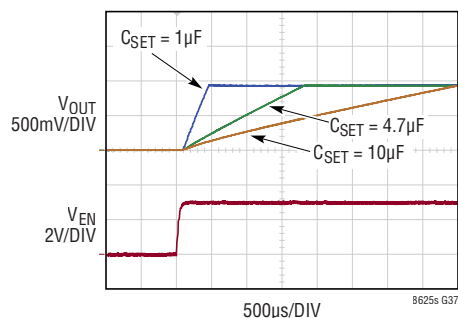
Soft-Start Waveforms
