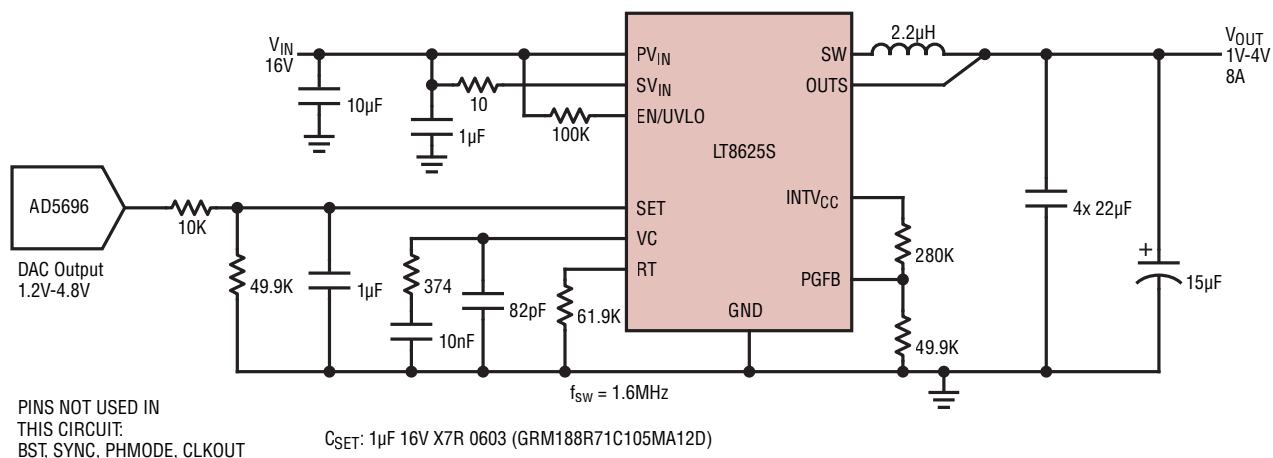
Dynamic Voltage Control 1V-4V 1.6MHz Step-Down Converter with External DAC
