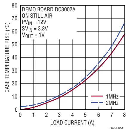
LT8625S Case Temperature Rise
