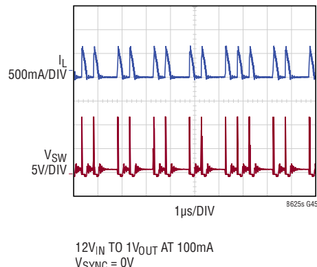
Switching Waveforms, Pulse-Skipping Operation
