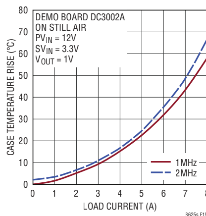
Figure 15. LT8625S Case Temperature Rise
