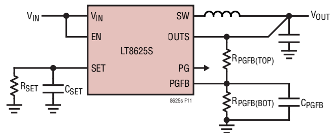
Figure 11. Figure 1. Schematic with C_{\text{PGFB}}
