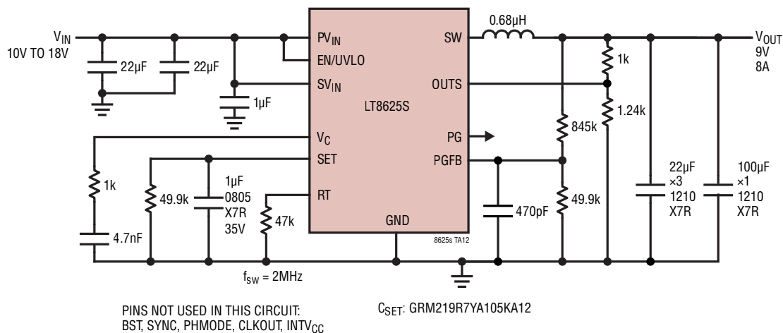
9V 8A 2MHz Step-Down Converter with Soft-Start, Fast Start-Up and Power Good
