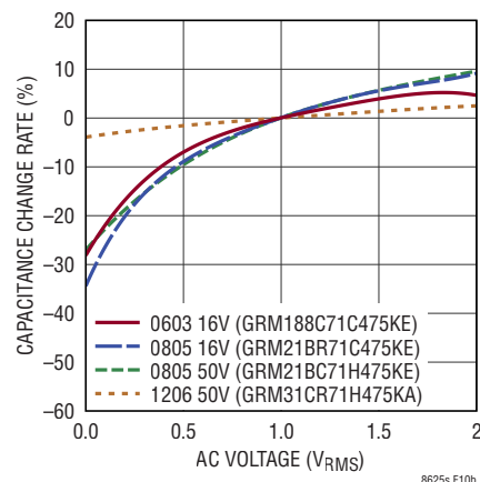
(b) Rated Capacitance = 4.7µF
