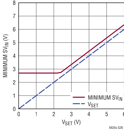
Minimum SV IN as a Function of V SET
