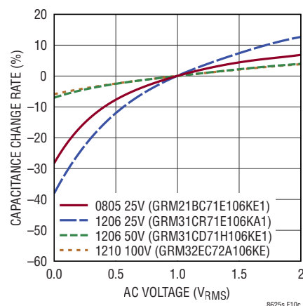
(c) Rated Capacitance = 10µF
