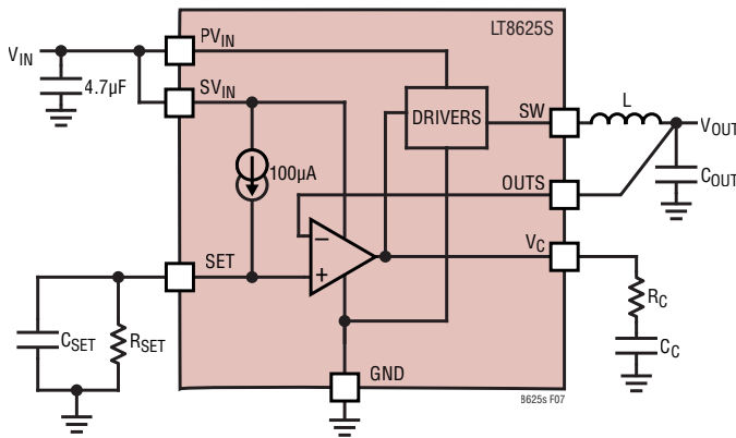
Figure 7. Adjustable Reference for Error Amplifier
