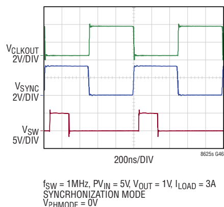
CLKOUT Waveforms
