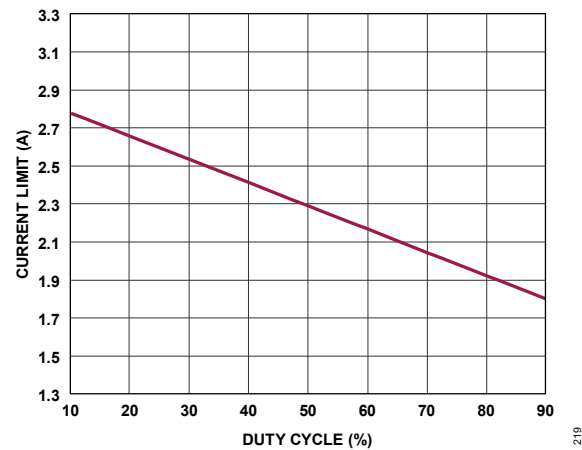
Figure 24. Top MOSFET Current Limit vs. Duty Cycle
