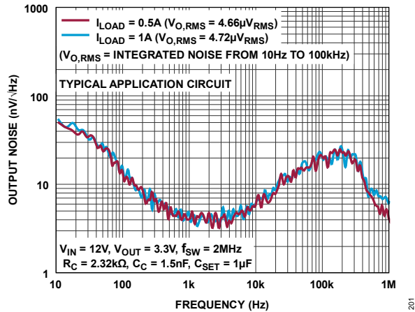
Figure 4. Noise Spectral Density vs. Load See Typical Application Circuit (Figure 62)
