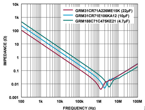
Figure 53. Frequency Characteristics of Example Output Capacitors for 2MHz Operation
