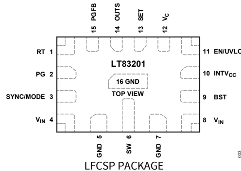
LFCSP PACKAGE
