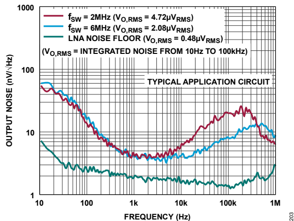
Figure 6. Noise Spectral Density vs. Switching Frequency See Typical Application Circuit (Figure 63)
