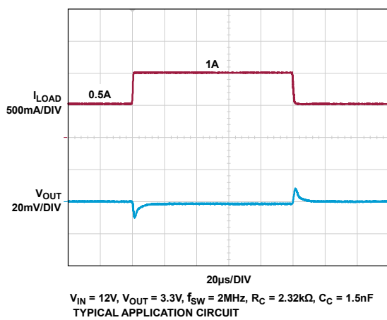
Figure 44. Transient Response: Load Current Stepped from 0.5A to 1A
