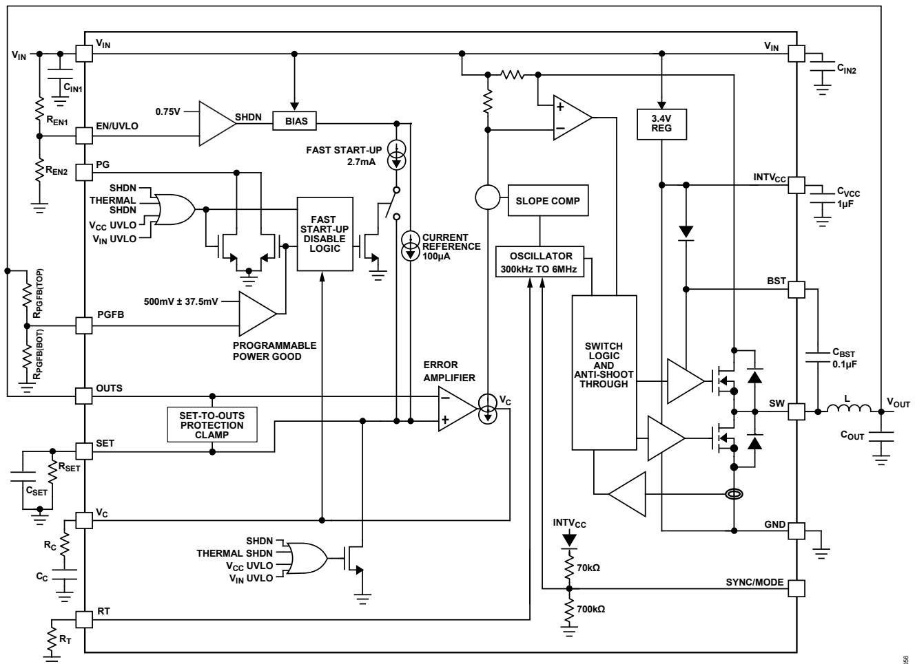
Figure 48. Block Diagram
