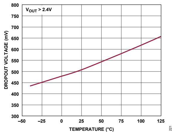
Figure 26. V_{IN} to V_{SET} Dropout Voltage vs. Temperature
