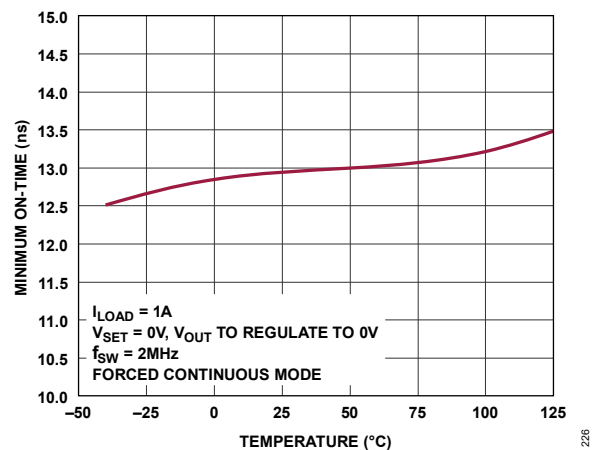
Figure 31. Minimum On-Time vs. Temperature
