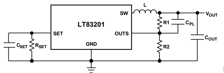
Figure 55. Configuring the LT83201 for Output Voltages above 13V
