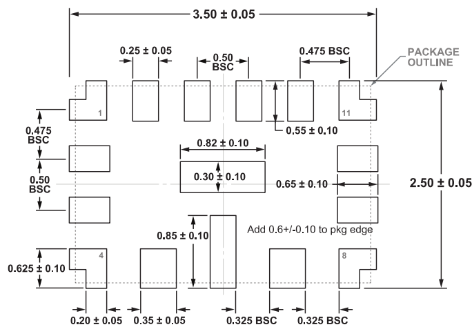
Figure 68. Tiny 15-Lead 3mm × 2mm LFCSP
