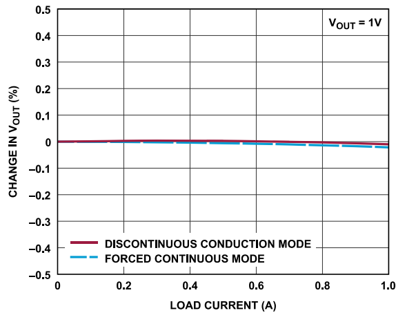
Figure 20. Load Regulation
