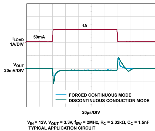
Figure 45. Transient Response: Load Current Stepped from 50mA to 1A
