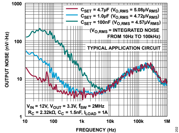
Figure 5. Noise Spectral Density vs. CSET See Typical Application Circuit (Figure 62)
