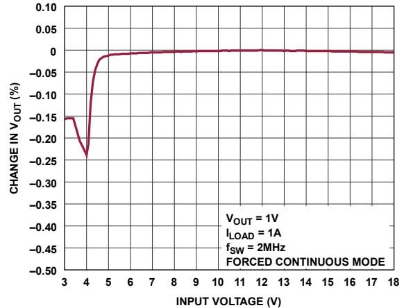
Figure 21. Line Regulation
