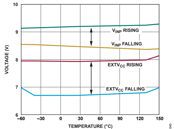
Figure 40. EXT_V_{CC} , V_{INP} , Switchover Thresholds for GATEV_{CC} Regulation
