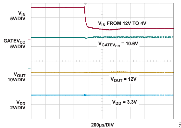
Figure 41. GATEV CC Response to Input Brownout (EXTV CC = 12V)
