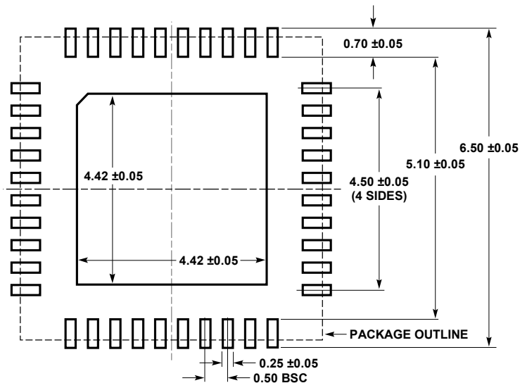
UJ Package 40-Lead Plastic QFN (6mm × 6mm) (Reference LTC DWG # 05-08-1728 Rev Ø)
