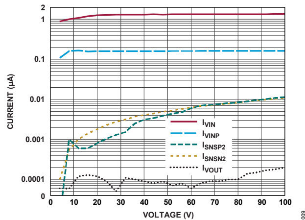
Figure 9. Shutdown Currents vs. Voltage
