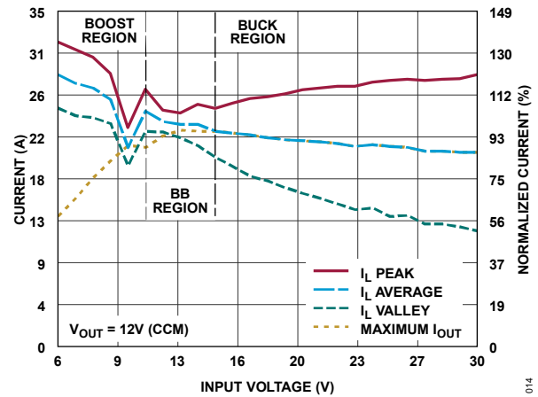
Figure 14. Maximum Inductor Current: f_{SW} = f_{SW(Optimal)} (Figure 79)
