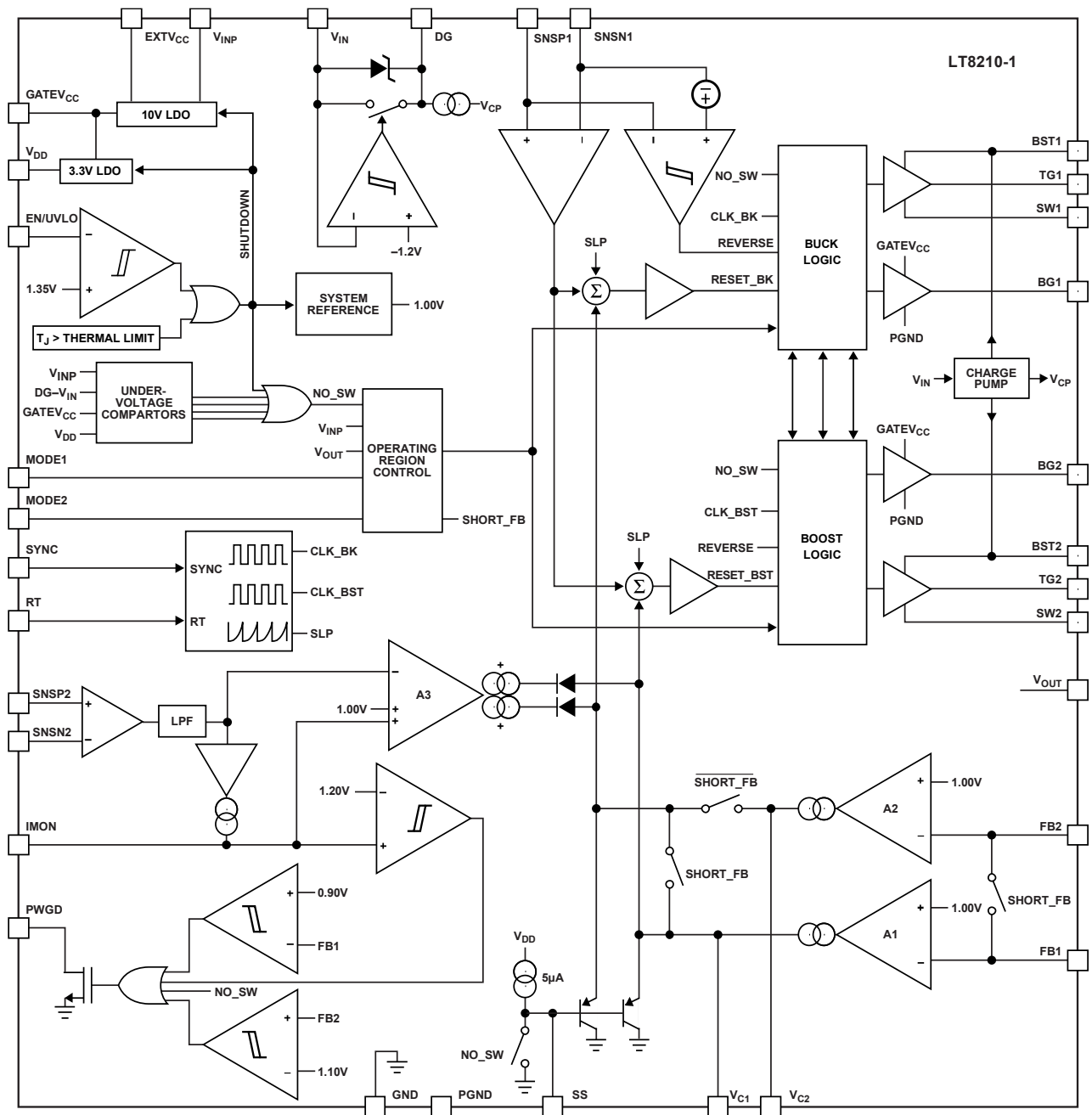
Figure 4. Block Diagram
