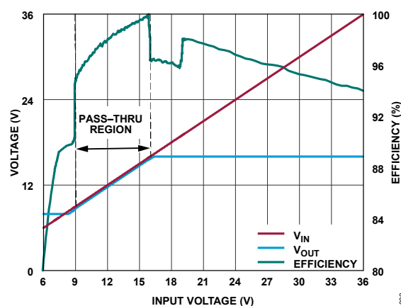
Figure 2. Pass-Thru Transfer Characteristic ( V_{OUT(BOOST)} = 8V , V_{OUT(BUCK)} = 16V ) 75A LOAD
