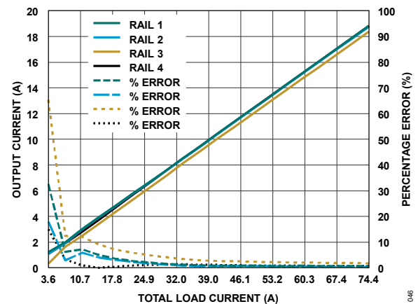
Figure 46. Current Sharing, 12V IN , CCM
