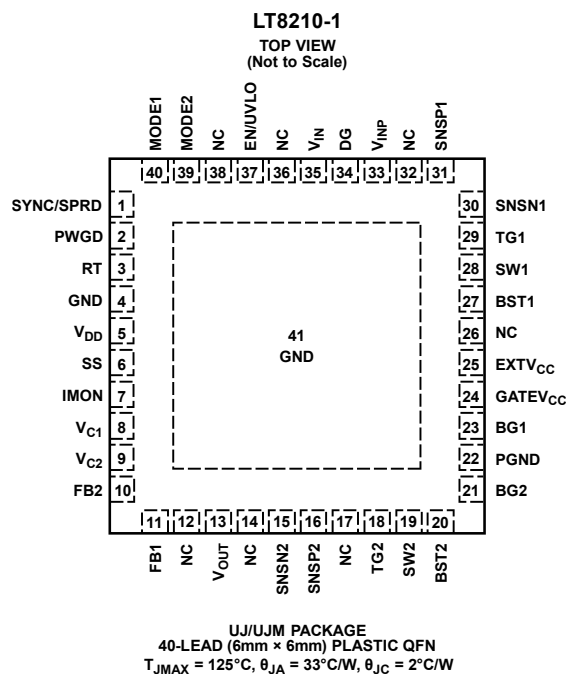
Figure 3. Pin Diagram
