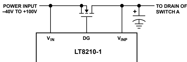
Figure 56. Implementing Reverse Input Protection
