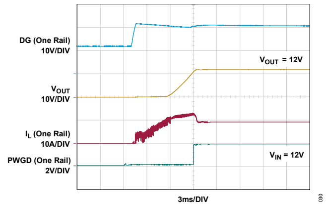
Figure 30. Pass-Thru Start-Up: V_{IN} in Pass-Thru Window (Figure 79)
