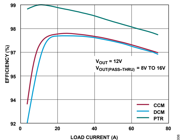
Figure 6. Efficiency vs. Load Current ( V_{IN} = 12V – Figure 79)
