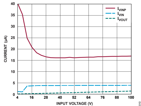
Figure 10. Pass-Thru Non-Switching Currents vs. Input Voltage
