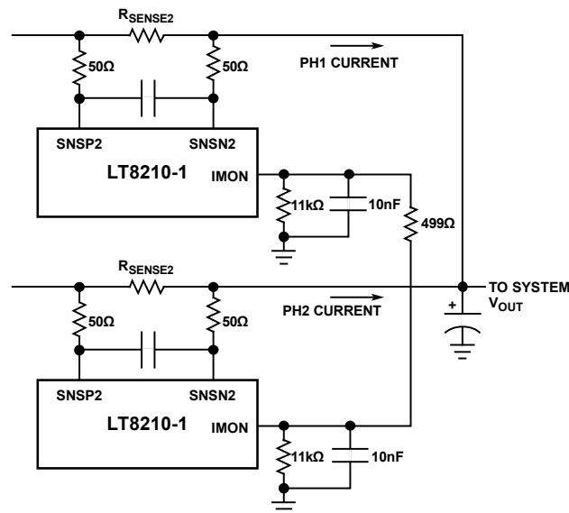
Figure 57. 2-Phase Current Sharing
