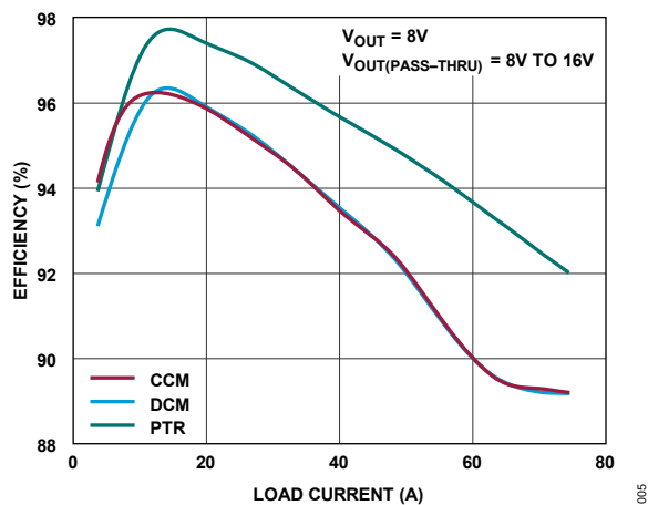
Figure 5. Efficiency vs. Load Current ( V_{IN} = 6V – Figure 79)
