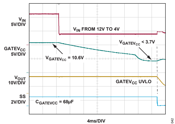
Figure 42. GATEV CC Response to Input Brownout (EXTV CC = 0V)
