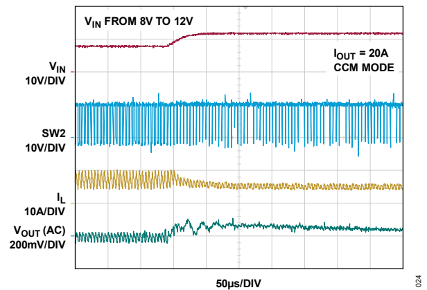
Figure 24. Line Step (Boost Region – Figure 79)
