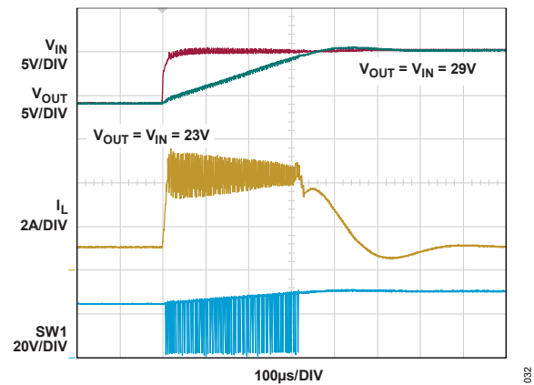
Figure 32. Pass-Thru Line Step (Figure 79)
