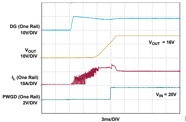
Figure 31. Pass-Thru Start-Up: V_{IN} above Pass-Thru Window (Figure 79)
