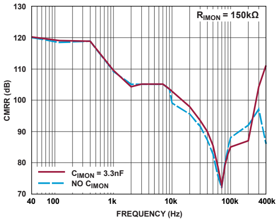
Figure 13. IMON CMRR vs. Frequency
