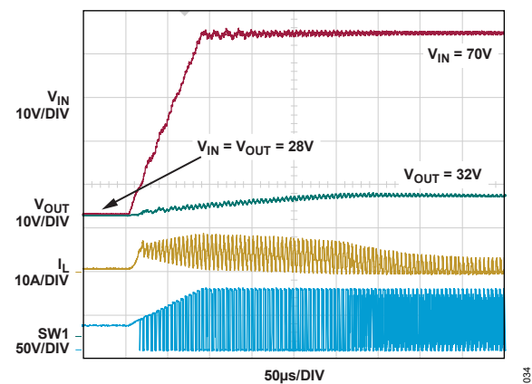
Figure 34. Pass-Thru Positive Surge (Figure 79)
