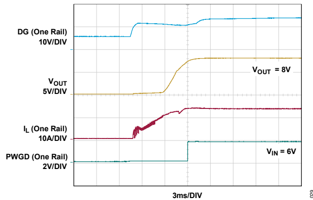
Figure 29. Pass-Thru Start-Up: V_{IN} Below Pass-Thru Window (Figure 79)
