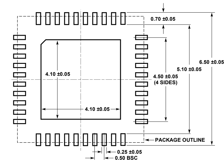
Figure 81. UJM Package Drawing
