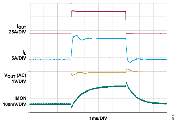
Figure 33. Pass-Thru Load Step (Figure 79)
