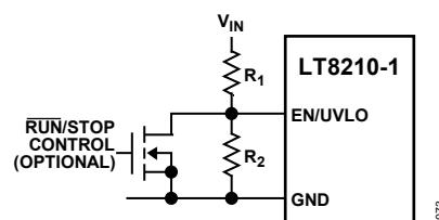
Figure 73. V_{IN} UVLO Implementation Using the EN/UVLO Pin
