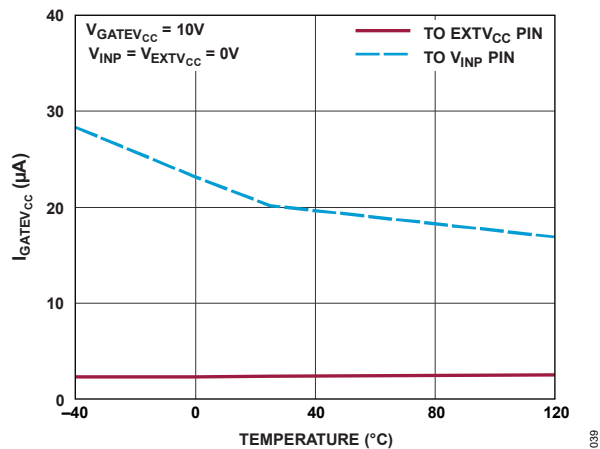
Figure 39. GATEV_{CC} Backdrive Current
