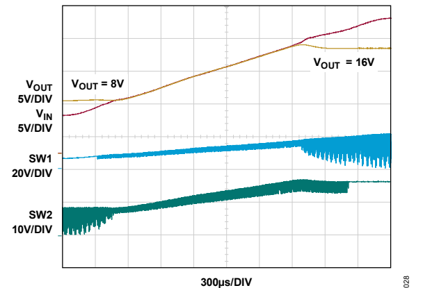
Figure 28. Input Voltage Sweep (Pass-Thru – Figure 79), 37.5A Load
