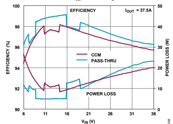
Figure 8. Efficiency and Power Loss vs. Input Voltage (Figure 79)
