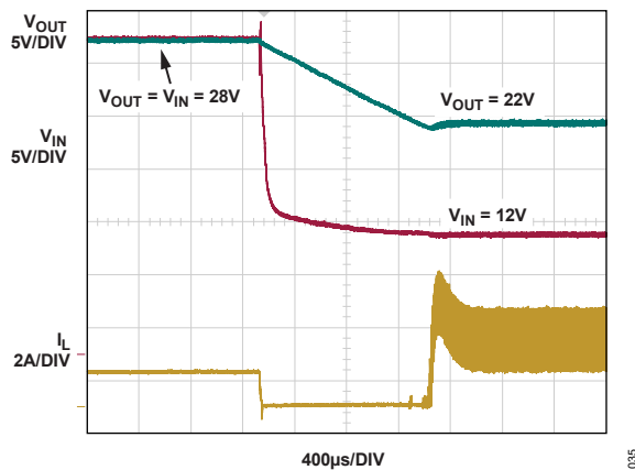
Figure 35. Pass-Thru Negative Surge (Figure 79)
