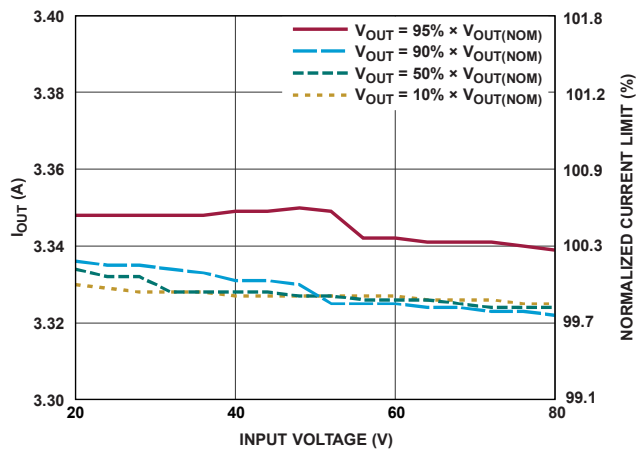
Figure 11. IMON Current Limit vs. Input Voltage (Figure 79)
