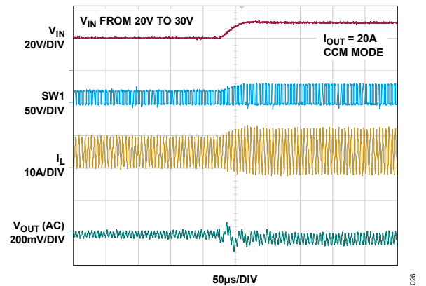
Figure 26. Line Step (Buck Region – Figure 79)
