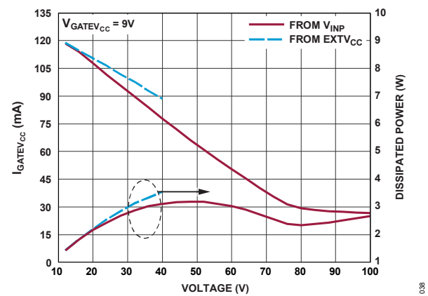
Figure 38. GATEV_{CC} Max Current vs. Voltage
