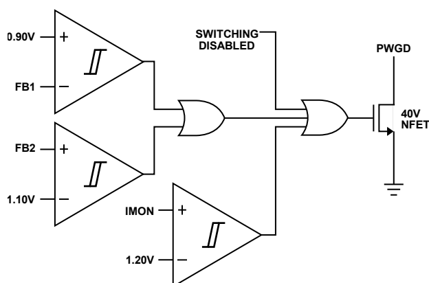
Figure 59. PWGD Logic
