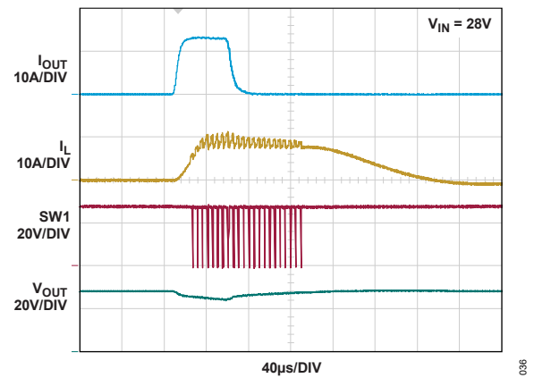
Figure 36. Pass-Thru Current Limit (Figure 79)
