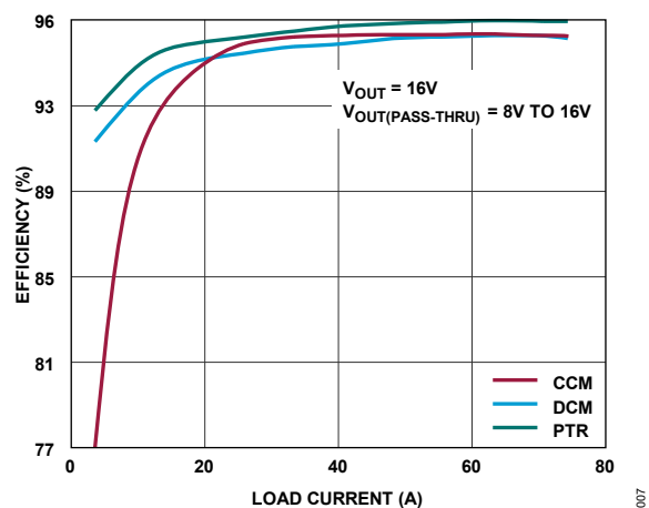
Figure 7. Efficiency vs. Load Current ( V_{IN} = 36V – Figure 79)
