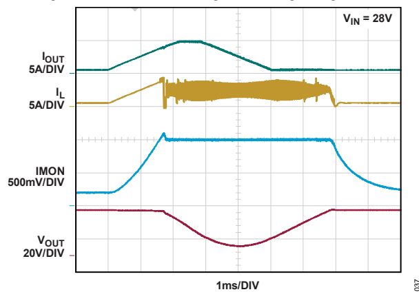
Figure 37. Pass-Thru IMON Limit (Figure 79)
