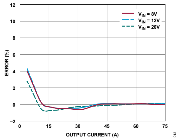
Figure 12. IMON Measurement Accuracy (Figure 79): V_{IN} = 8V , DCM
