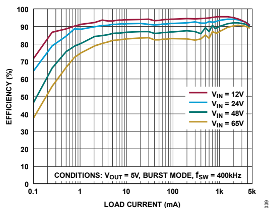
Figure 39. LT80603A Efficiency vs. Load Current
