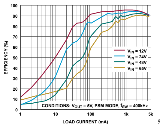
Figure 40. LT80603A Efficiency vs. Load Current
