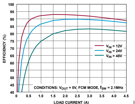
Figure 41. LT80603A Efficiency vs. Load Current
