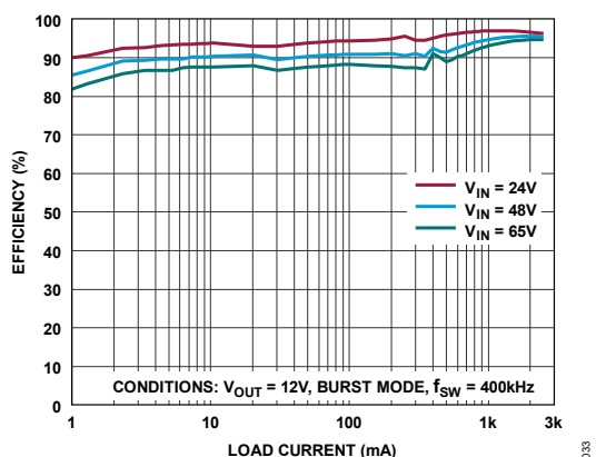
Figure 33. LT80602 Efficiency vs. Load Current
