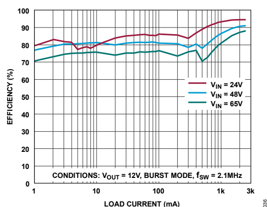
Figure 36. LT80602 Efficiency vs. Load Current
