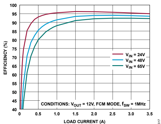
Figure 17. LT80603 Efficiency vs. Load Current
