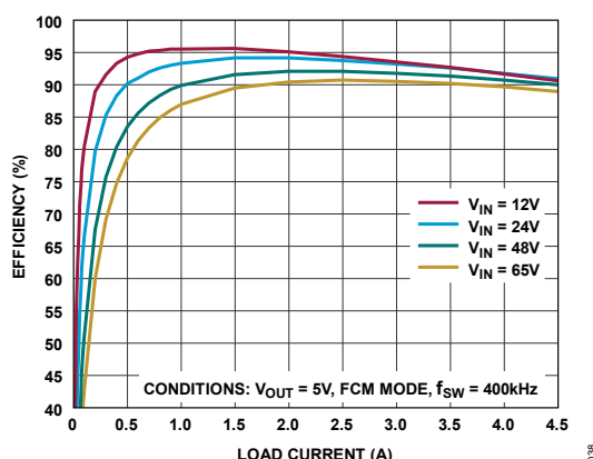
Figure 38. LT80603A Efficiency vs. Load Current
