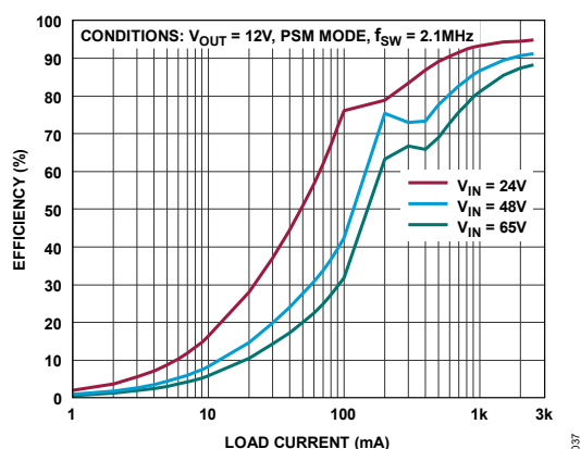
Figure 37. LT80602 Efficiency vs. Load Current
