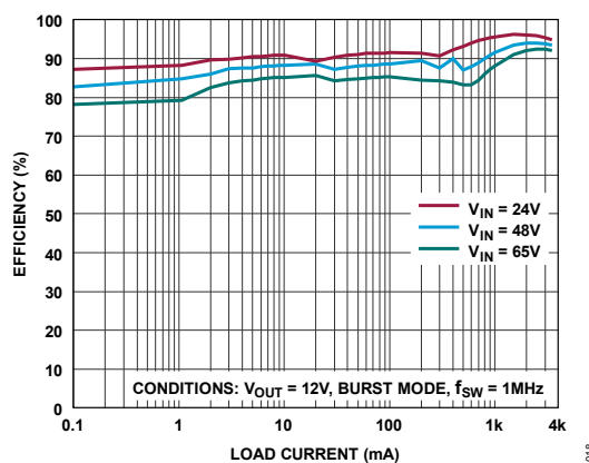
Figure 18. LT80603 Efficiency vs. Load Current
