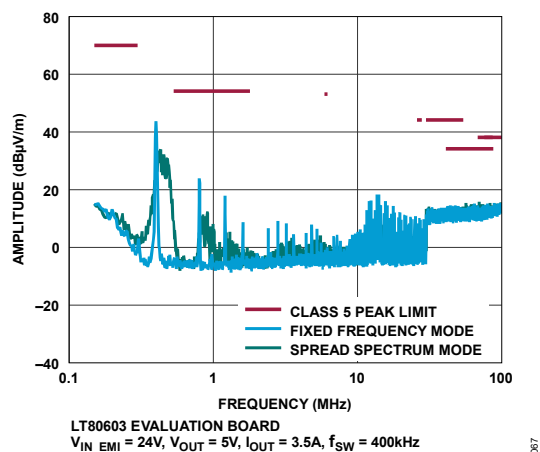
Figure 67. LT80603 CISPR 25 Conducted Emission Test with Class 5 Peak Limits (See Figure 89, Typical Application Circuit)
