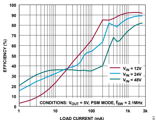
Figure 31. LT80602 Efficiency vs. Load Current
