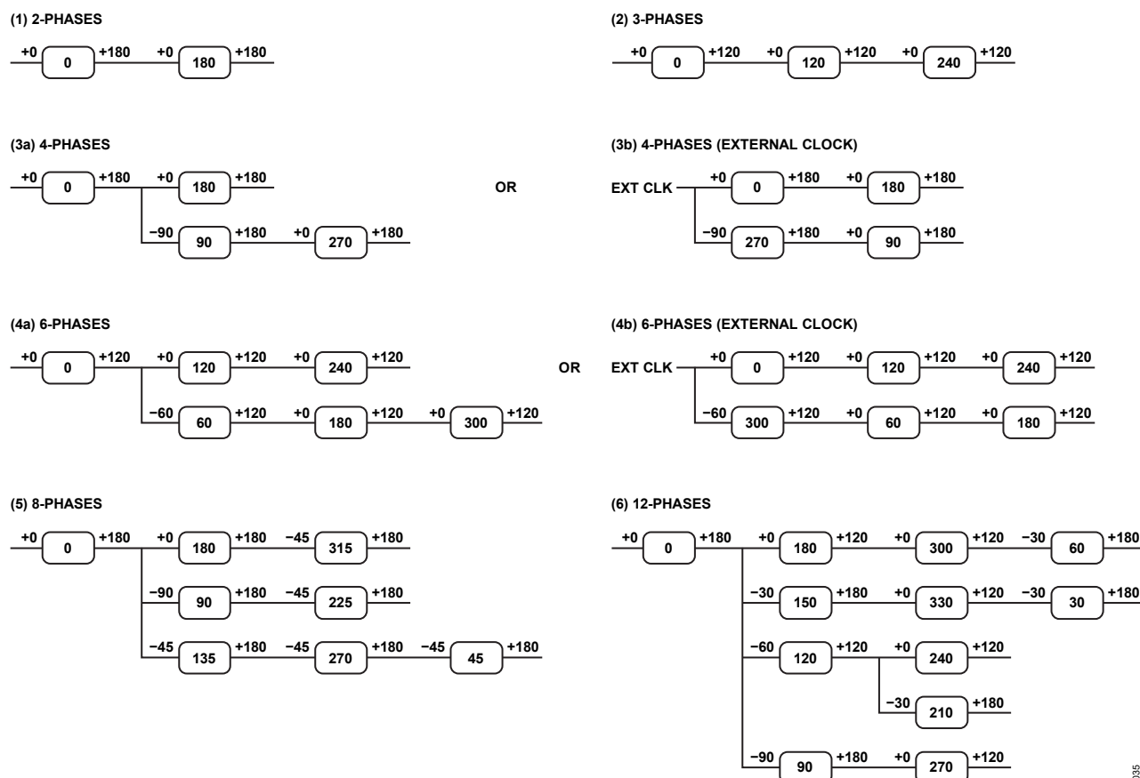
Figure 28. 2, 3, 4, 6, 8, 12 Multiphase Configuration
