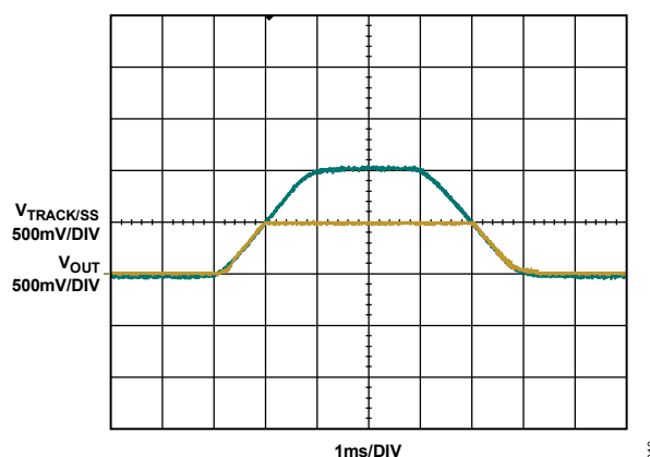
Figure 13. Output Tracking
