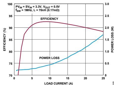
Figure 2. Efficiency and Power Loss (1MHz)
