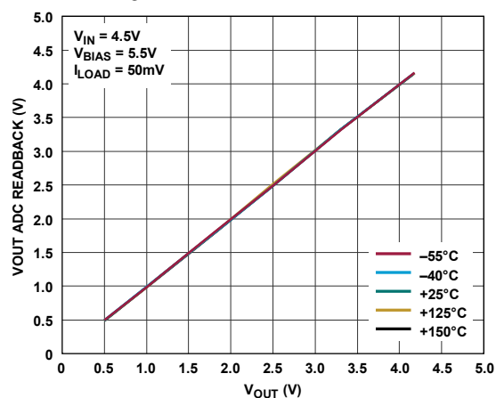
Figure 78. V_{OUT} ADC Readback
