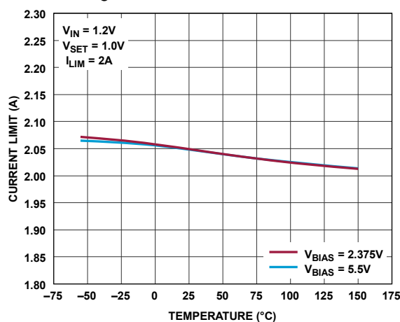
Figure 45. Programmable ILIM at 2A
