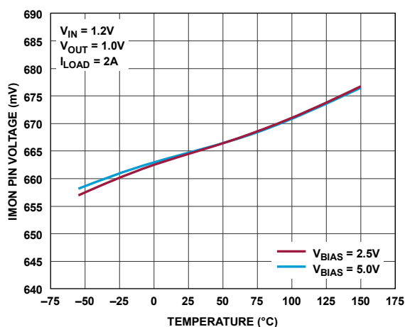
Figure 41. IMON Pin Voltage
