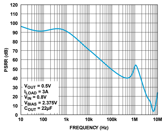
Figure 56. IN Pin PSRR
