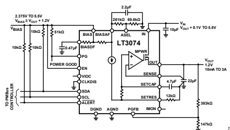
Figure 1. Simplified Application Diagram
