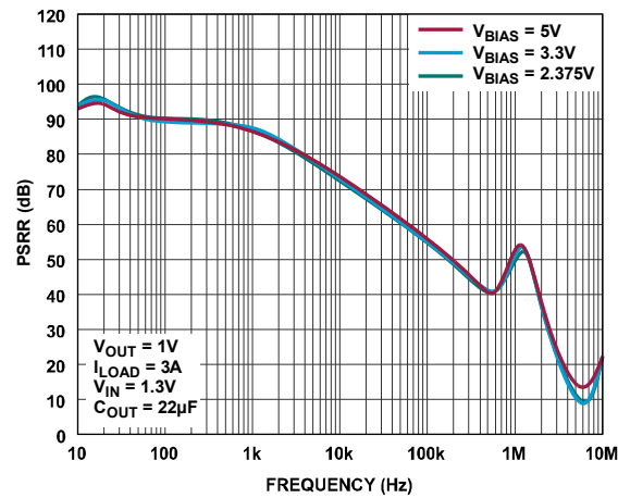
Figure 54. IN Pin PSRR
