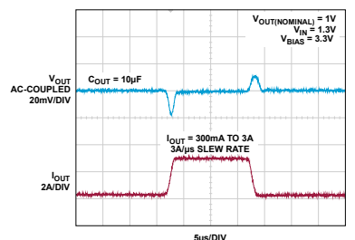
Figure 2. Transient Response
