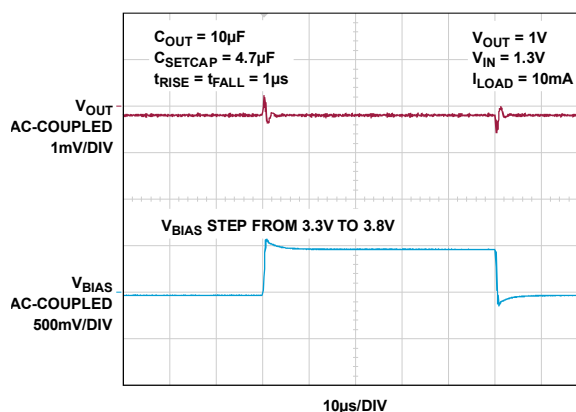
Figure 77. BIAS Line Transient Response
