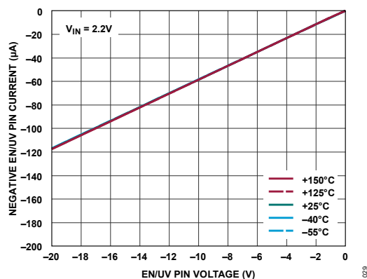
Figure 29. Negative EN/UV Pin Current vs. EN/UV Pin Voltage
