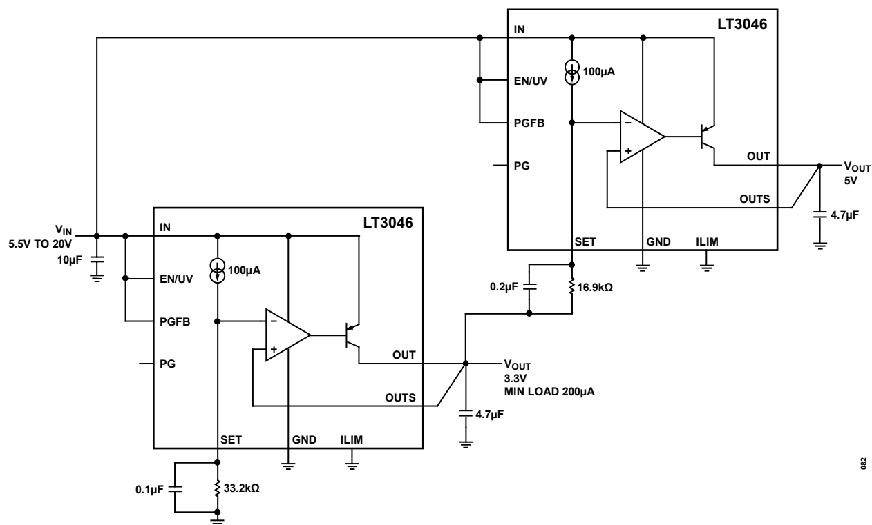
Figure 83. Ratiometric Tracking
