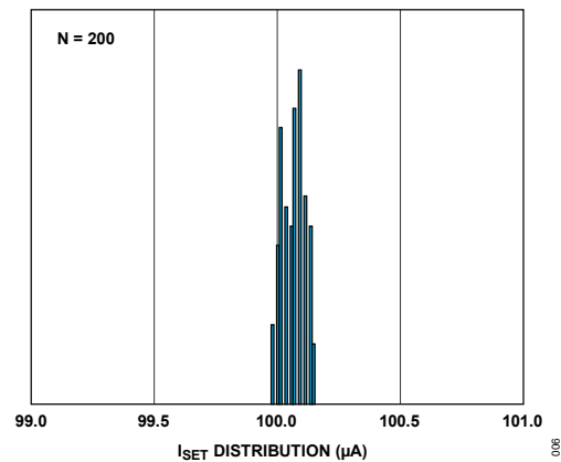
Figure 6. I_{SET} Distribution
