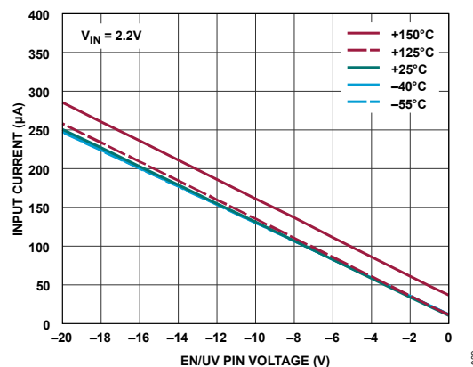
Figure 30. Input Current vs. EN/UV Pin Voltage
