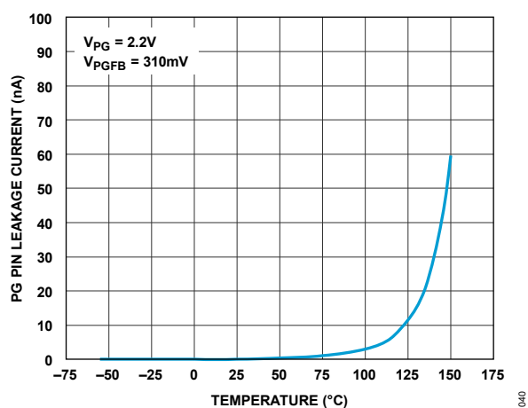
Figure 40. PG Pin Leakage Current vs. Temperature
