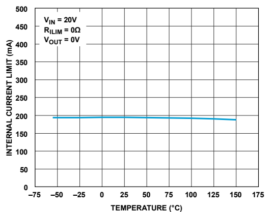
Figure 32. Internal Current Limit vs. Temperature (Foldback)
