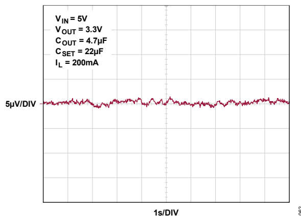
Figure 62. Output Noise: 0.1Hz to 10Hz ( C_{SET} = 22\mu\text{F} )
