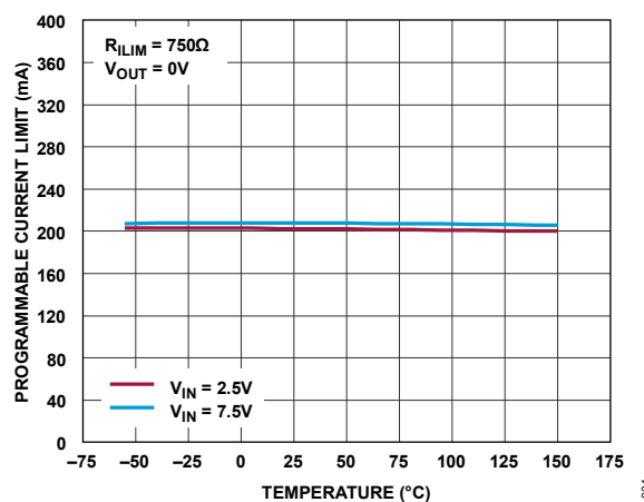
Figure 34. Programmable Current Limit vs. Temperature (200mA)
