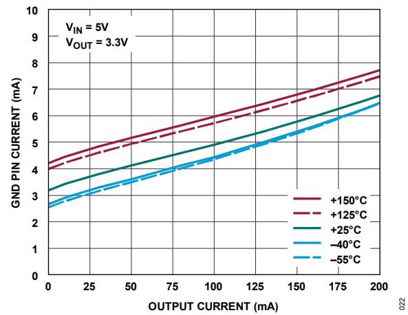
Figure 22. GND Pin Current vs. Output Current
