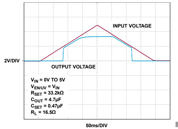
Figure 66. Input Supply Ramp-Up and Ramp-Down
