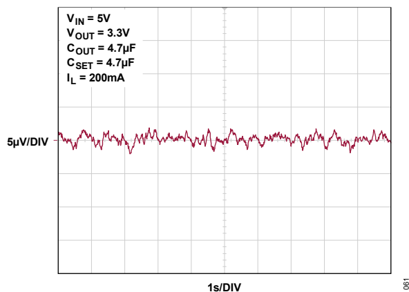
Figure 61. Output Noise: 0.1Hz to 10Hz ( C_{SET} = 4.7\mu\text{F} )
