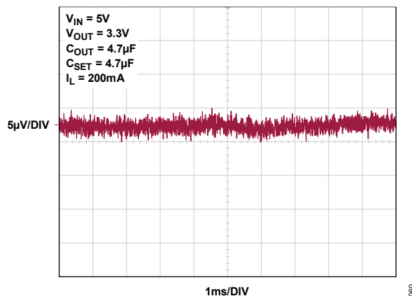
Figure 60. Output Noise: 10Hz to 100kHz
