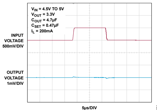
Figure 64. Line-Transient Response
