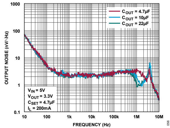
Figure 56. Output Noise vs. Frequency ( C_{OUT} Steps)
