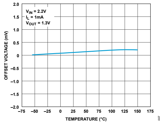
Figure 7. Offset Voltage ( V_{OUT} - V_{SET} ) vs. Temperature
