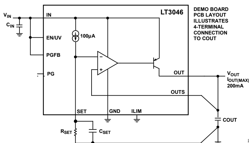
Figure 70. C OUT and C SET Connections for Best Performance
