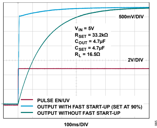
Figure 65. Start-Up Time With and Without Fast Start-Up Circuitry for Large C_{SET}
