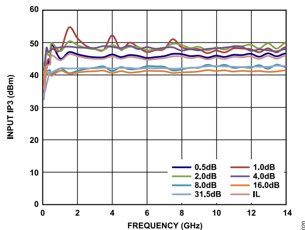
Figure 21. Input IP3 vs. Frequency over Major Attenuation States, V_{EE} = -5\text{ V}
