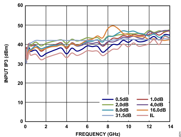
Figure 22. Input IP3 vs. Frequency over Major Attenuation States, V_{EE} = -3\text{ V}
