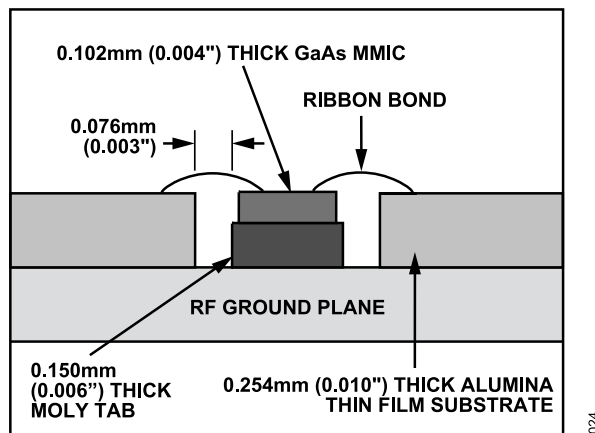
Figure 25. Bonding RF Pads to 10 mil Substrate
