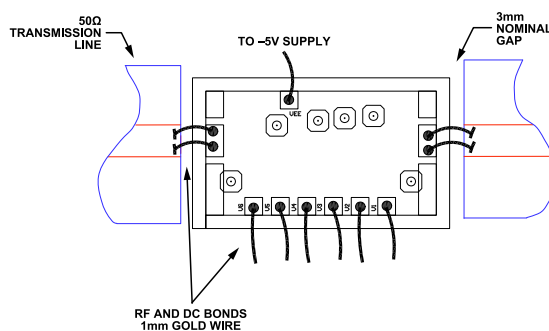
Figure 26. Assembly Diagram
