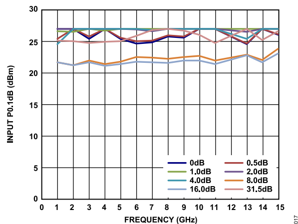
Figure 18. Input P0.1dB vs. Frequency over Major Attenuation States, V_{EE} = -5\text{ V}
