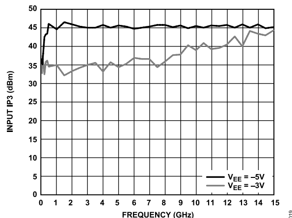
Figure 20. Input IP3 vs. Frequency at Minimum Attenuation State over V_{EE} = -5\text{ V} and V_{EE} = -3\text{ V}
