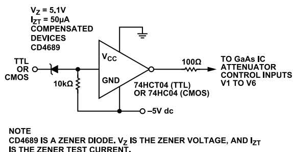
Figure 23. Suggested Driver Circuit
