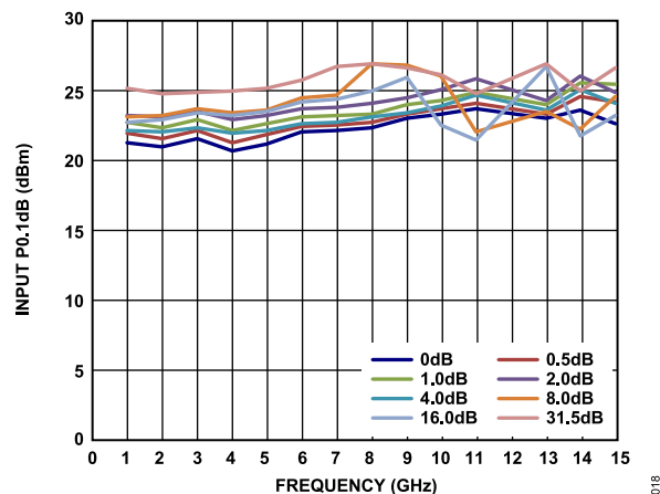
Figure 19. Input P0.1dB vs. Frequency over Major Attenuation States, V_{EE} = -3\text{ V}
