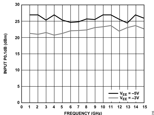
Figure 17. Input P0.1dB vs. Frequency at Minimum Attenuation State over V_{EE} = -5\text{ V} and V_{EE} = -3\text{ V}
