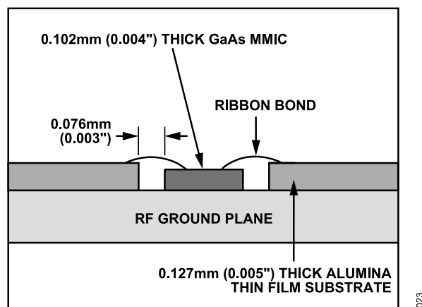
Figure 24. Bonding RF Pads to 5 mil Substrate
