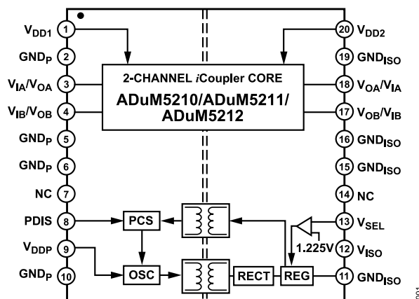
Figure 1. ADuM5210/ADuM5211/ADuM5212
