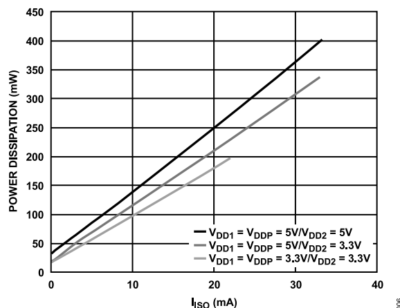
Figure 7. Typical Total Power Dissipation vs. I_{ISO}
