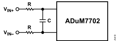
Figure 29. Differential RC Filter Network
