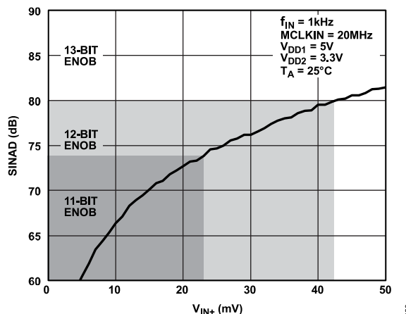
Figure 27. SINAD vs. V_{IN+} AC Input Signal Amplitude
