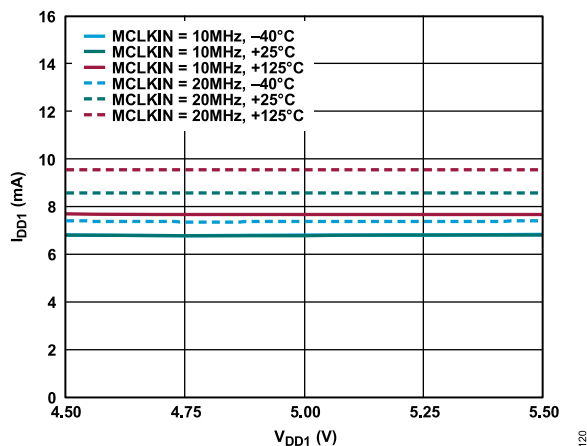
Figure 19. I_{DD1} vs. V_{DD1} at Clock Rates and Various Temperatures
