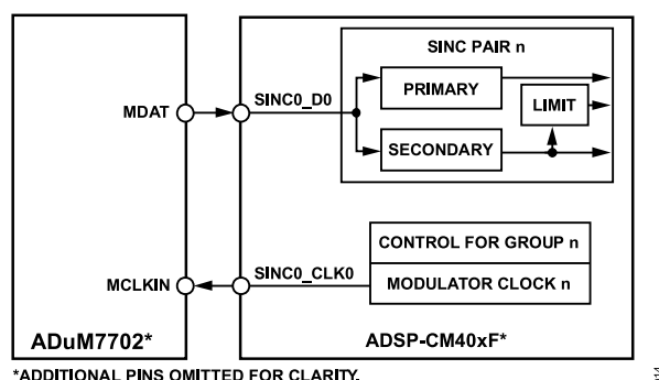
Figure 31. Interfacing the ADuM7702 to the ADSP-CM4xx
