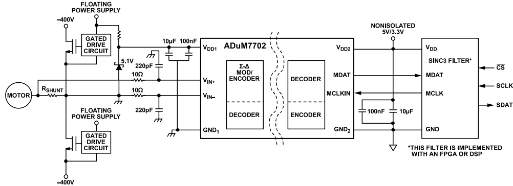
Figure 24. Typical Application Circuit
