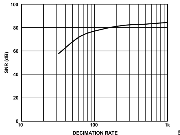
Figure 30. SNR vs. Decimation Rate of Sinc3 Filter Order
