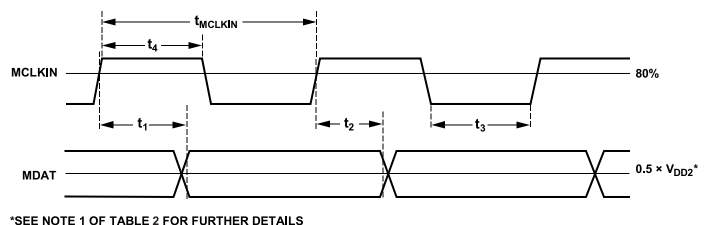
Figure 2. Data Timing Diagram
