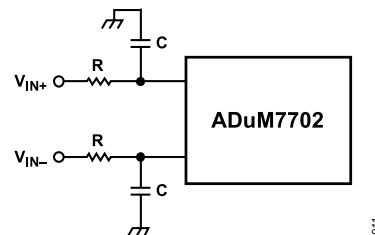
Figure 28. RC Low-Pass Filter Input Network
