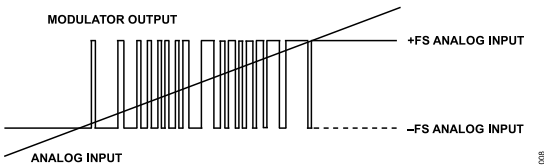
Figure 25. Analog Input vs. Modulator Output
