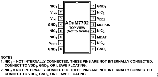
Figure 4. 16-Lead SOIC_W Pin Configuration
