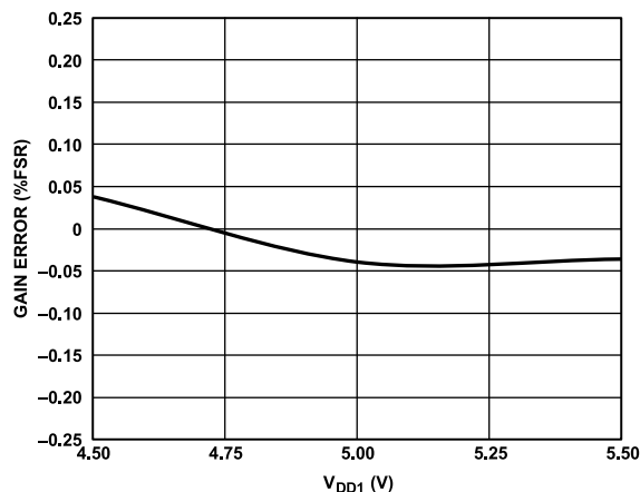
Figure 18. Gain Error vs. V_{DD1}
