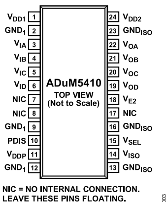
Figure 3. ADuM5410 Pin Configuration
