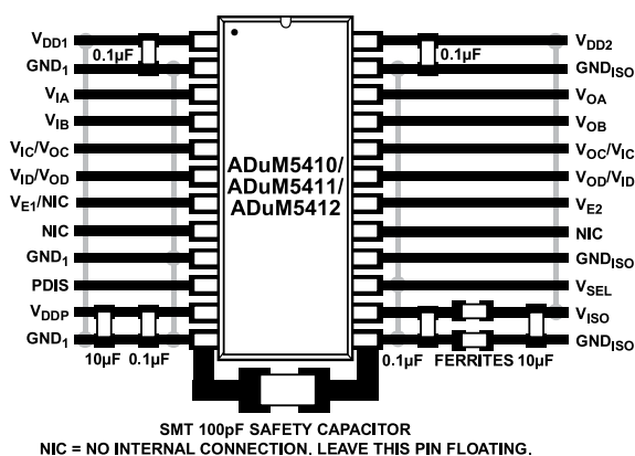
Figure 32. Recommended PCB Layout
