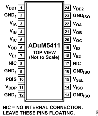
Figure 4. ADuM5411 Pin Configuration
