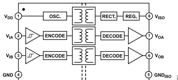
Figure 1. ADuM5240
