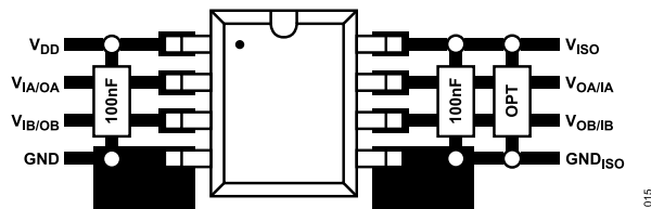
Figure 15. Recommended Printed Circuit Board Layout
