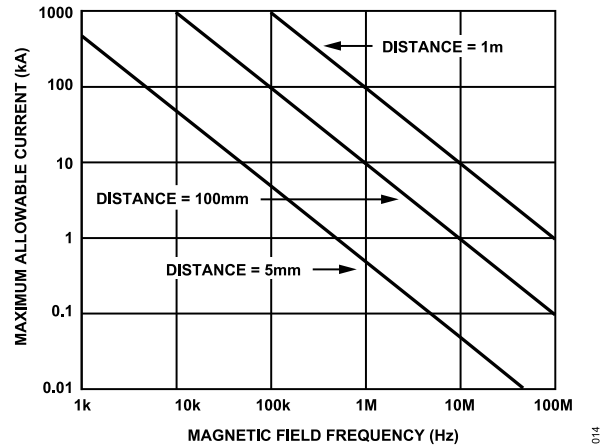
Figure 14. Maximum Allowable Current for Various Current-to-ADuM524x Spacings
