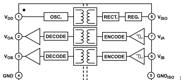
Figure 3. ADuM5242
