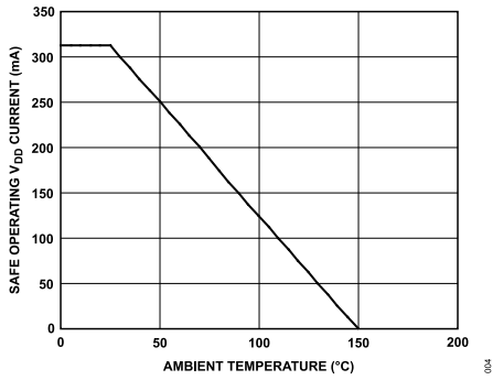
Figure 4. Thermal Derating Curve, Dependence of Safety-Limiting Values on Case Temperature, per DIN V VDE V 0884-17
