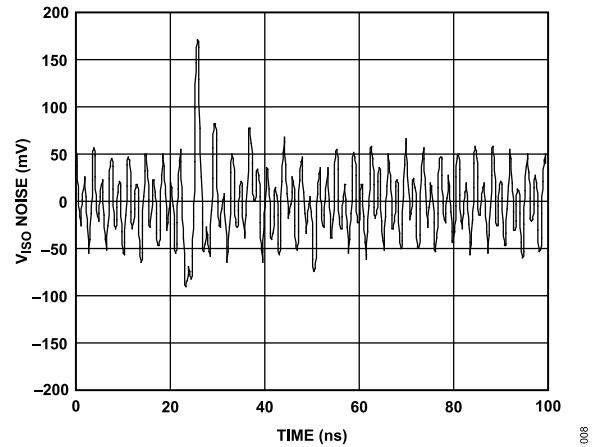
Figure 11. Typical Output Voltage Noise at 100% Load, 100 nF Bypass Capacitance vs. Time
