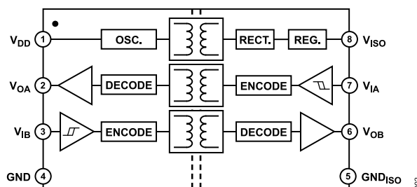
Figure 2. ADuM5241
