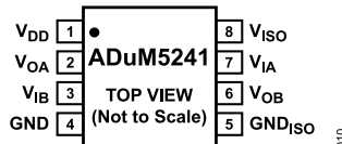
Figure 6. ADuM5241 Pin Configuration
