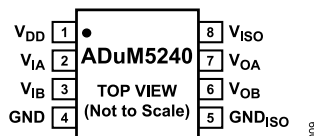
Figure 5. ADuM5240 Pin Configuration
