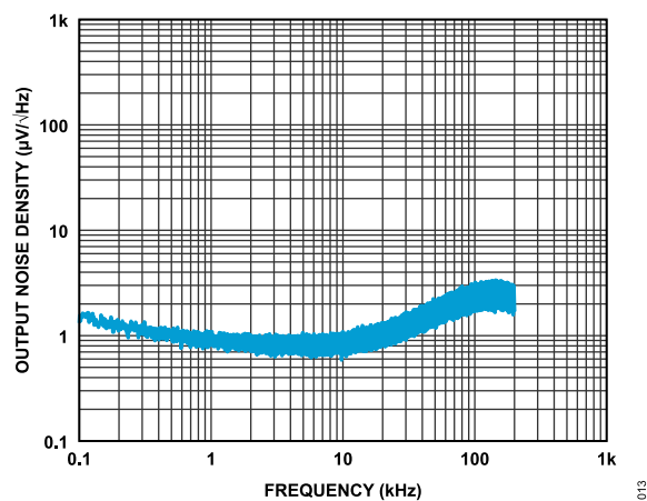
Figure 13. Output Noise Density vs. Frequency
