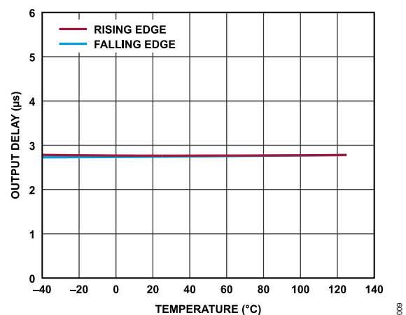
Figure 9. Output Delay vs. Temperature
