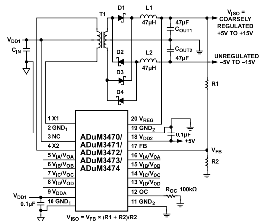
Figure 40. Positive Supply and Unregulated Negative Supply
