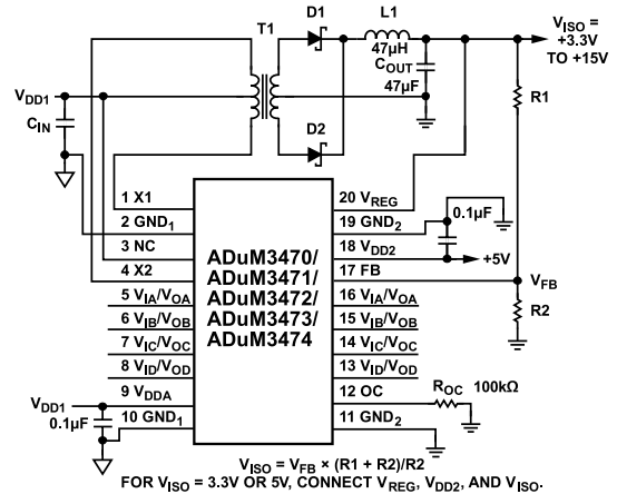
Figure 38. Single Power Supply
