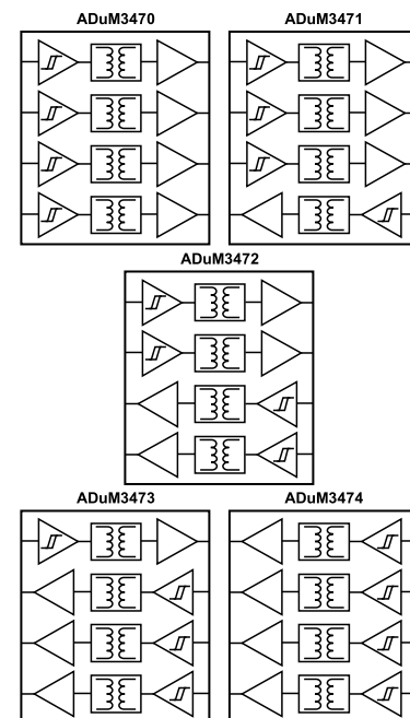
Figure 2. Block Diagrams of I/O Channels
