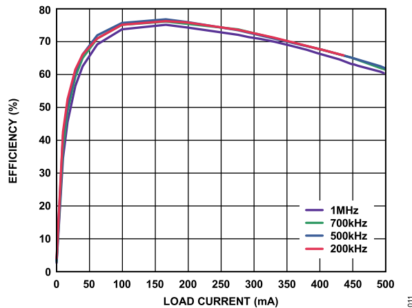
Figure 11. Typical Efficiency at Various Switching Frequencies with Halo Transformer, 5 V Input to 5 V Output
