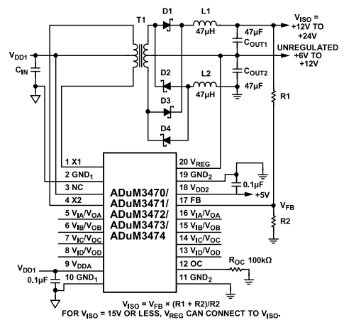
Figure 39. Doubling Power Supply
