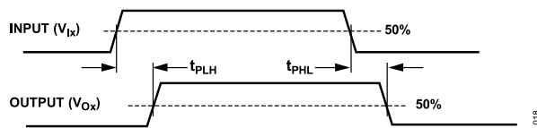
Figure 42. Propagation Delay Parameters
