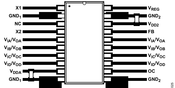
Figure 41. Recommended PCB Layout
