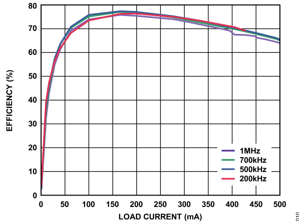
Figure 10. Typical Efficiency at Various Switching Frequencies with Coilcraft Transformer, 5 V Input to 5 V Output
