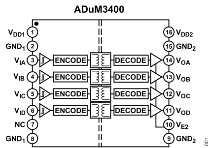
Figure 1. ADuM3400 Functional Block Diagram
