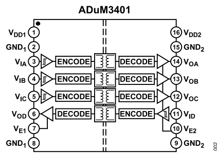
Figure 2. ADuM3401 Functional Block Diagram
