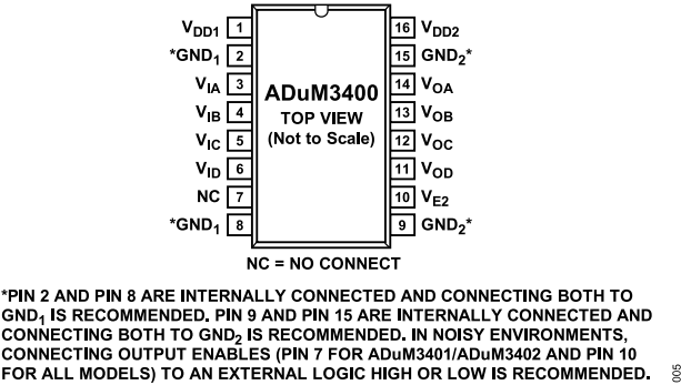
Figure 5. ADuM3400 Pin Configuration
