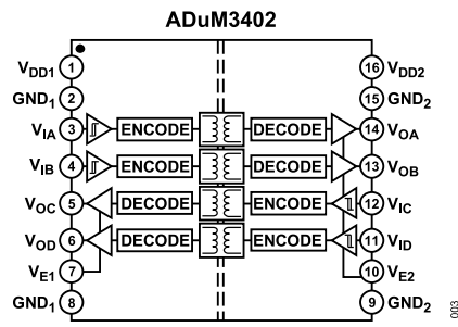
Figure 3. ADuM3402 Functional Block Diagram
