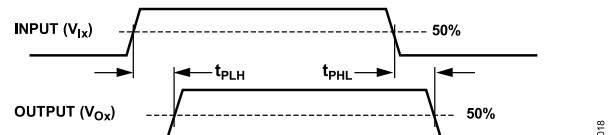
Figure 18. Propagation Delay Parameters
