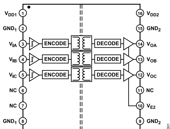
Figure 1. ADuM3300 Functional Block Diagram
