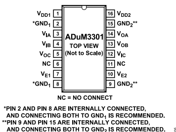
Figure 5. ADuM3301 Pin Configuration
