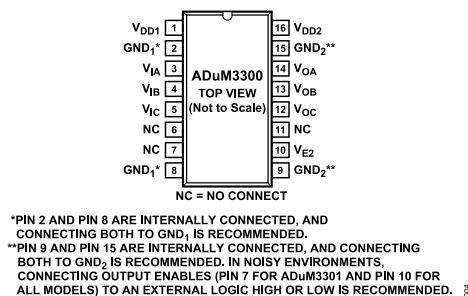
Figure 4. ADuM3300 Pin Configuration
