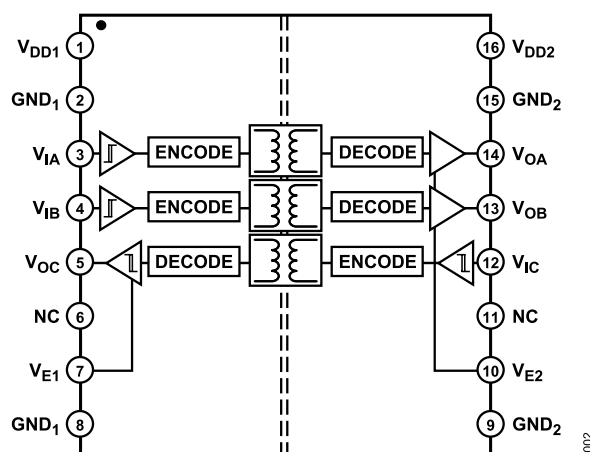
Figure 2. ADuM3301 Functional Block Diagram
