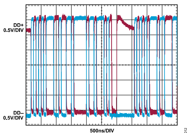
Figure 13. Full Speed Data (Downstream, DD+ and DD-)
