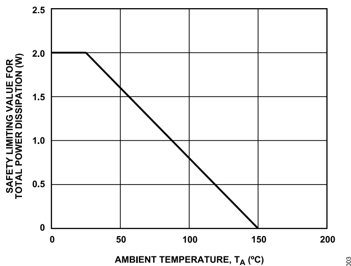
Figure 3. Thermal Derating Curve, Dependence of Safety Limiting Values with Ambient Temperature per VDE 0884-17
