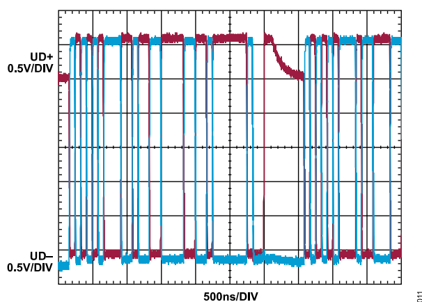
Figure 16. Full Speed Data (Upstream, UD+ and UD-)
