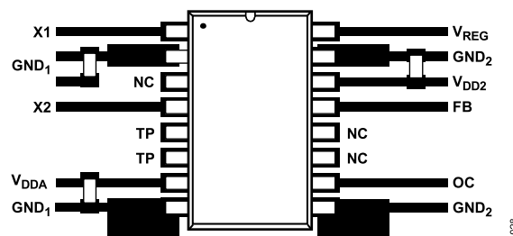
Figure 34. Recommended PCB Layout
