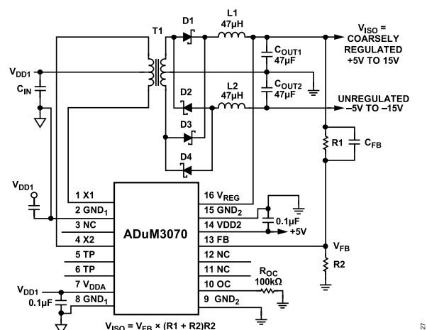
Figure 33. Positive and Unregulated Negative Supply
