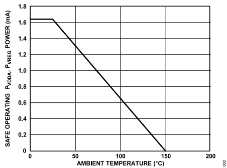
Figure 2. Thermal Derating Curve, Dependence of Safety Limiting Values on Ambient Temperature, per DIN EN IEC 60747-17 (VDE 0884-17)
