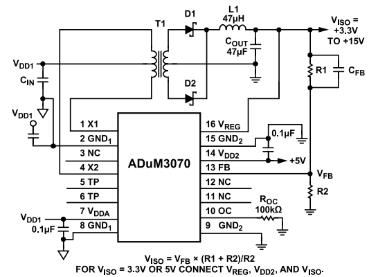
Figure 31. Single Power Supply
