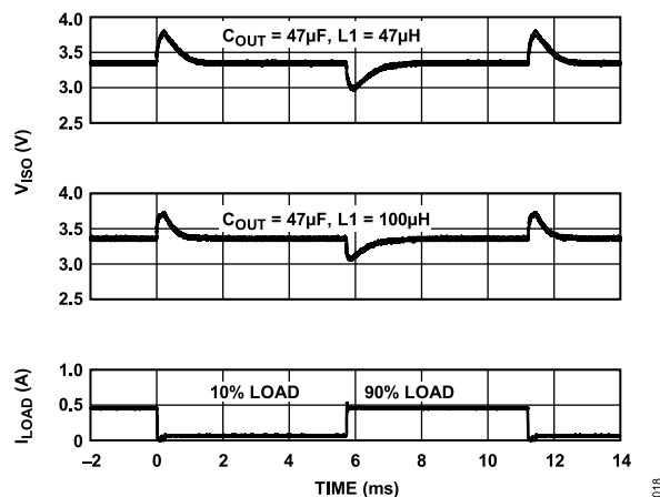
Figure 21. Typical V_{ISO} Load Transient Load Response, 5 V In to 3.3 V Out at 10% to 90% Load of 500 mA Load at 500 kHz f_{SW}
