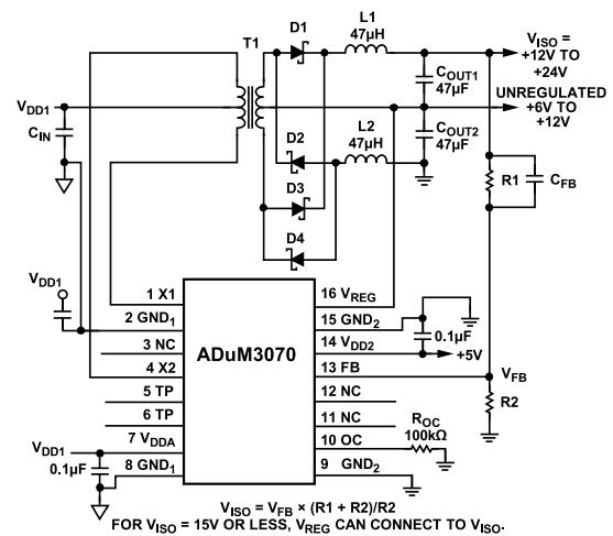
Figure 32. Doubling Power Supply
