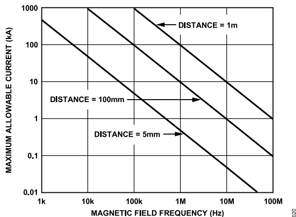
Figure 20. Maximum Allowable Current for Various Current-to-ADuM1100 Spacings
