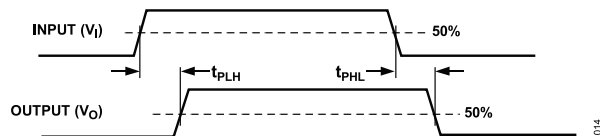
Figure 14. Propagation Delay Parameters
