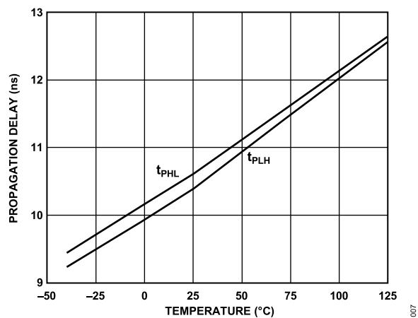
Figure 7. Typical Propagation Delays vs. Temperature, 5 V Operation
