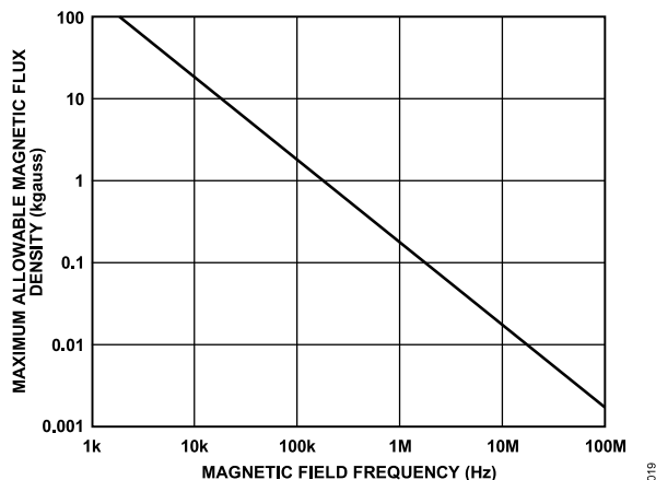
Figure 19. Maximum Allowable External Magnetic Field
