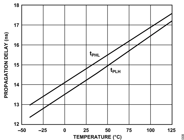
Figure 8. Typical Propagation Delays vs. Temperature, 3.3 V Operation
