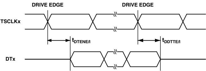
Figure 21. Enable and Three-State
