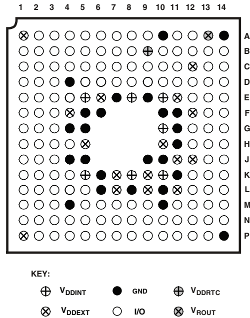
Figure 62. 182-Ball CSP_BGA Configuration (Top View)
