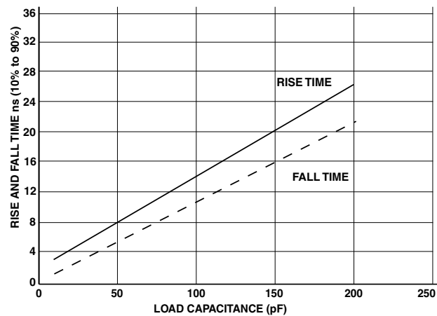
Figure 59. Typical Output Delay or Hold for Driver E at V_{DDEXT} Max
