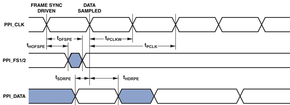
Figure 15. PPI GP Rx Mode with Internal Frame Sync Timing
