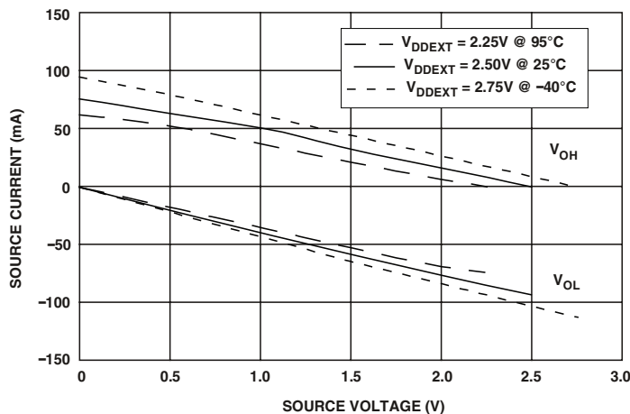
Figure 37. Drive Current B (Low V_{DDEXT} )
