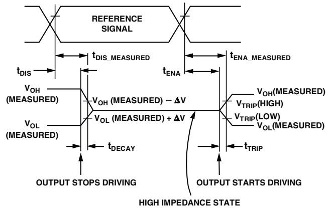
Figure 48. Output Enable/Disable
