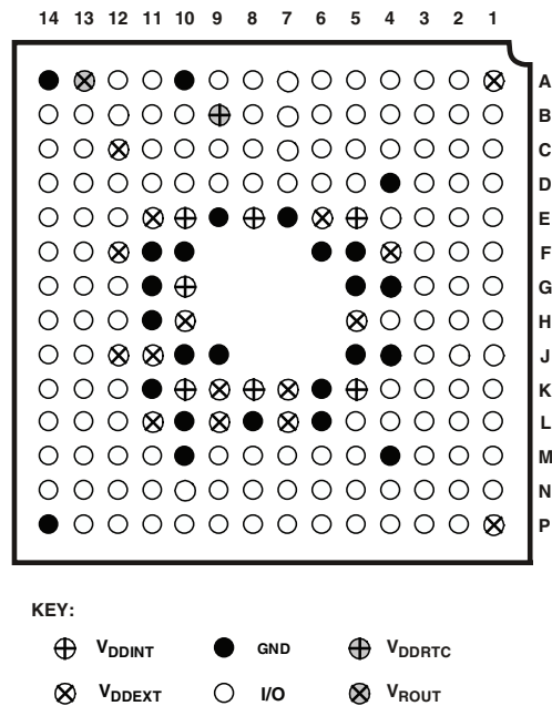
Figure 63. 182-Ball CSP_BGA Configuration (Bottom View)
