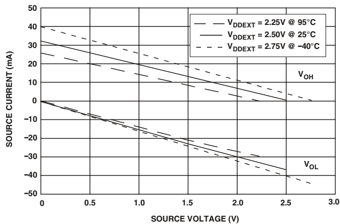
Figure 43. Drive Current E (Low V_{DDEXT} )
