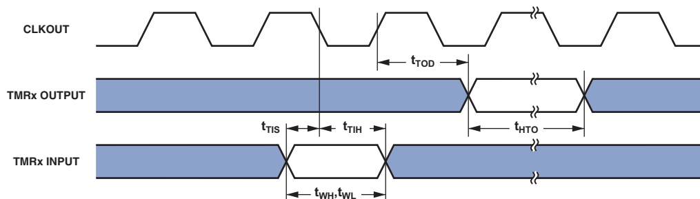
Figure 27. Timer Cycle Timing
