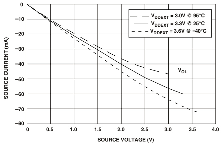
Figure 46. Drive Current F (High V_{DDEXT} )
