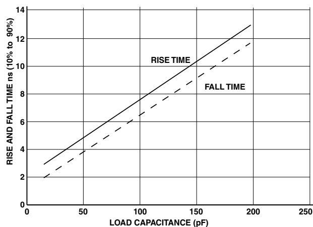
Figure 57. Typical Output Delay or Hold for Driver D at V_{DDEXT} \text{ Max}
