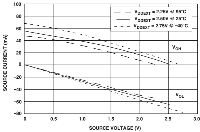
Figure 41. Drive Current D (Low V_{DDEXT} )
