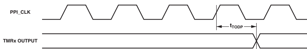
Figure 26. Timer Clock Timing
