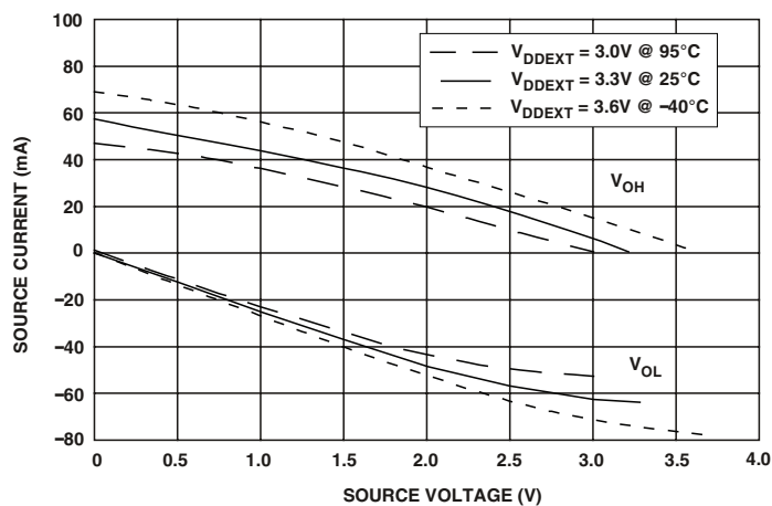
Figure 40. Drive Current C (High V_{DDEXT} )
