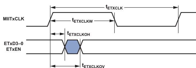
Figure 30. 10/100 Ethernet MAC Controller Timing: MII Transmit Signal
