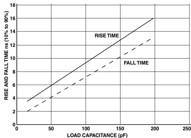
Figure 56. Typical Output Delay or Hold for Driver D at V_{DDEXT} \text{ Min}
