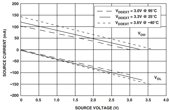
Figure 38. Drive Current B (High V_{DDEXT} )
