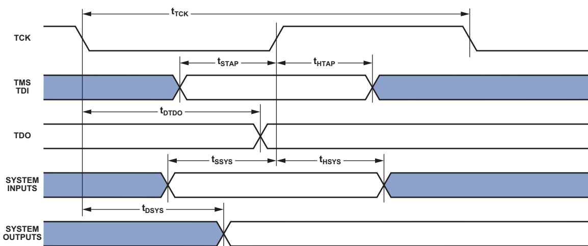
Figure 28. JTAG Port Timing
