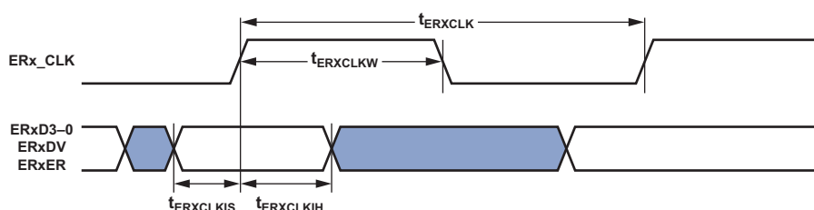
Figure 29. 10/100 Ethernet MAC Controller Timing: MII Receive Signal
