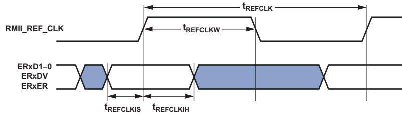
Figure 31. 10/100 Ethernet MAC Controller Timing: RMII Receive Signal
