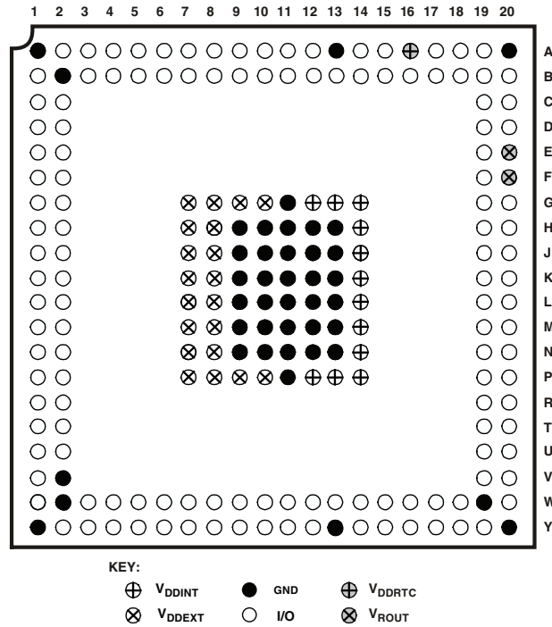
Figure 64. 208-Ball CSP_BGA Configuration (Top View)
