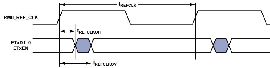
Figure 32. 10/100 Ethernet MAC Controller Timing: RMII Transmit Signal
