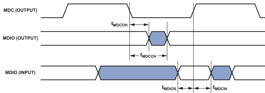
Figure 34. 10/100 Ethernet MAC Controller Timing: MII Station Management
