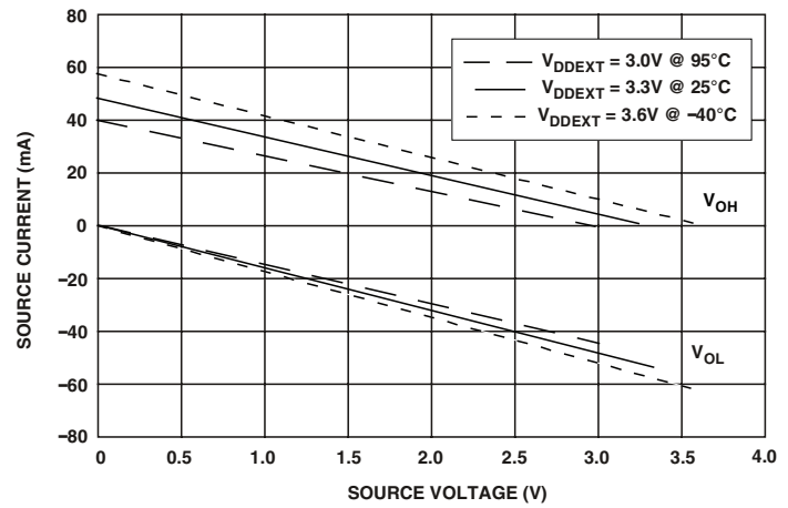
Figure 44. Drive Current E (High V_{DDEXT} )
