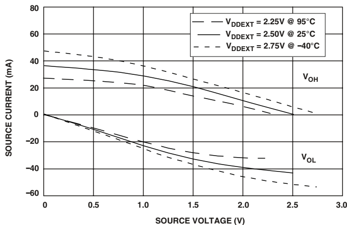
Figure 39. Drive Current C (Low V_{DDEXT} )
