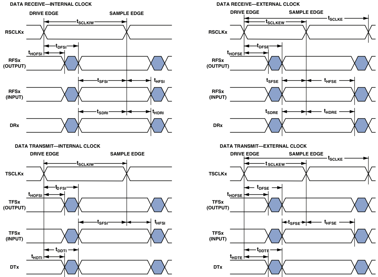
Figure 19. Serial Ports
