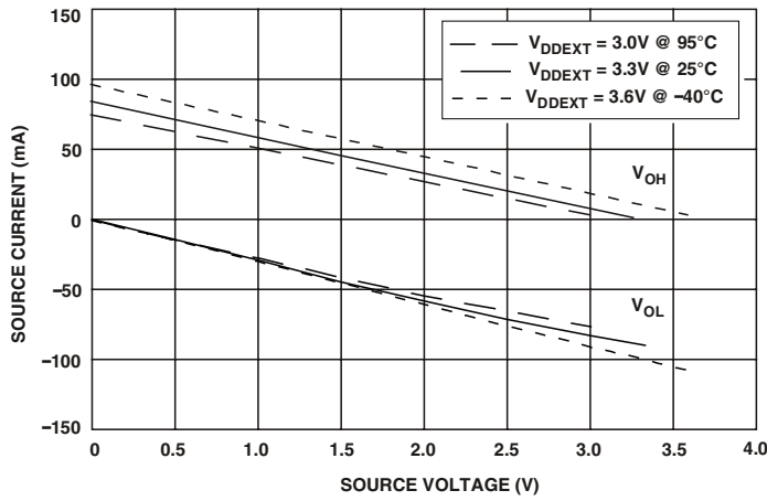
Figure 42. Drive Current D (High V_{DDEXT} )
