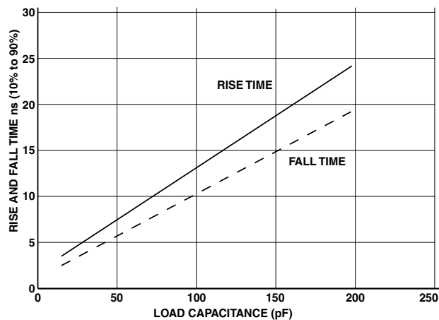
Figure 54. Typical Output Delay or Hold for Driver C at V_{DDEXT} \text{ Min}
