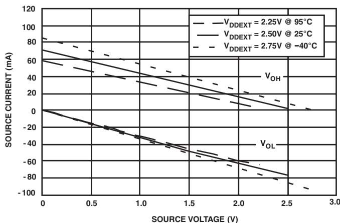
Figure 35. Drive Current A (Low V_{DDEXT} )
