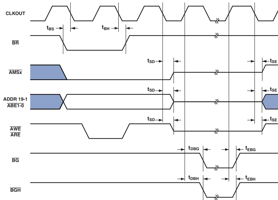
Figure 12. External Port Bus Request and Grant Cycle Timing
