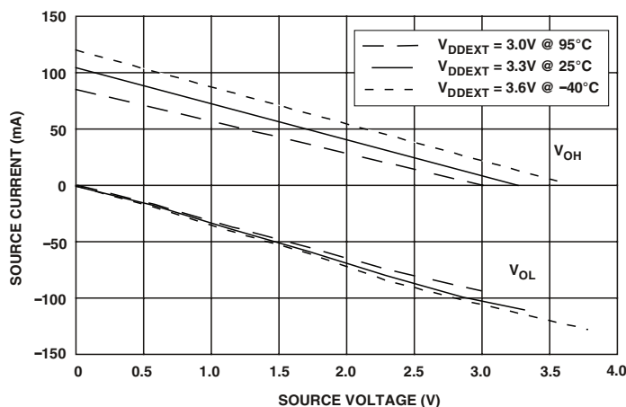
Figure 36. Drive Current A (High V_{DDEXT} )
