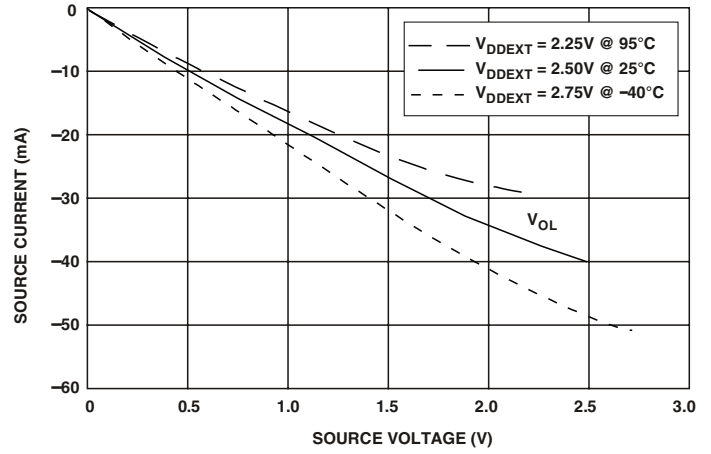
Figure 45. Drive Current F (Low V_{DDEXT} )
