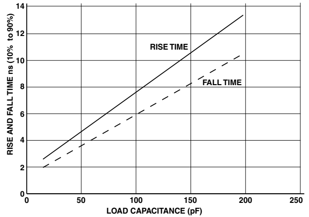
Figure 50. Typical Output Delay or Hold for Driver A at V_{DDEXT} Min
