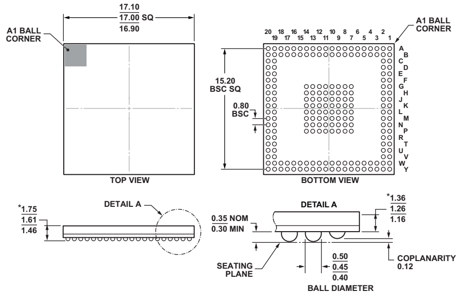
Figure 66. 182-Ball Chip Scale Package Ball Grid Array [CSP_BGA] (BC-182)
