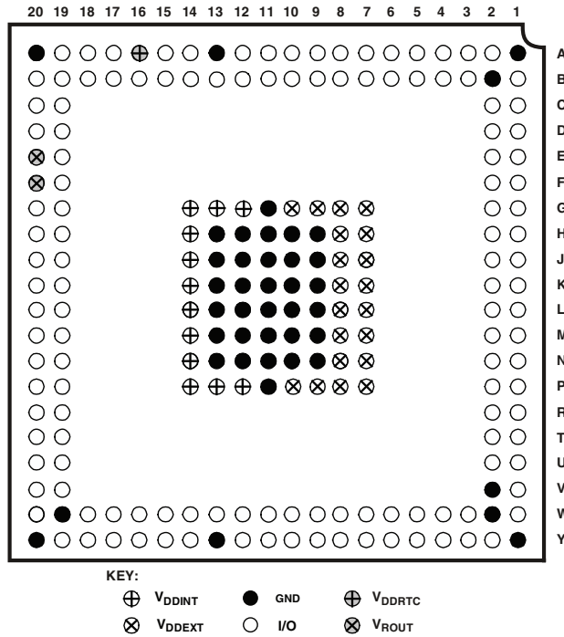
Figure 65. 208-Ball CSP_BGA Configuration (Bottom View)
