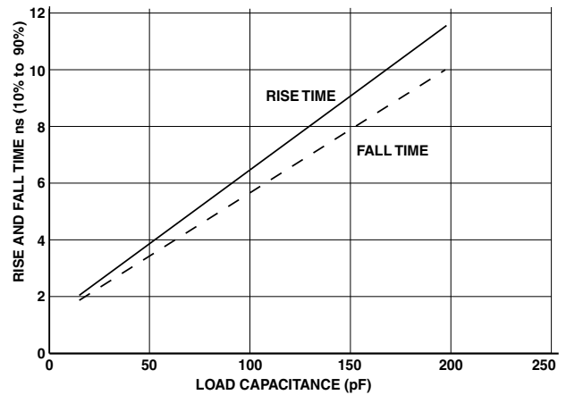
Figure 51. Typical Output Delay or Hold for Driver A at V_{DDEXT} Max
