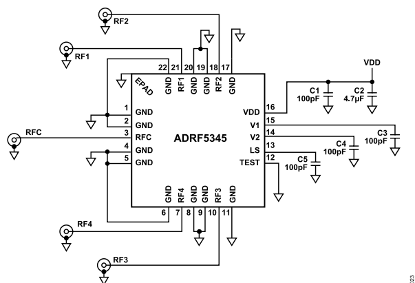
Figure 25. Recommended Schematic
