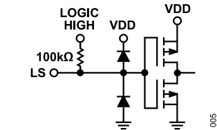
Figure 7. LS Control Interface Schematic
