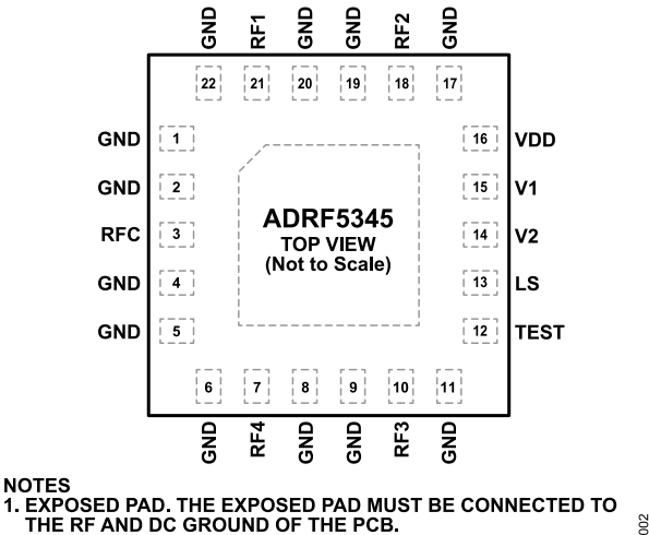
Figure 4. Pin Configuration
