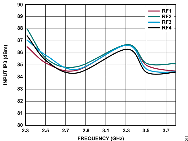
Figure 20. Input IP3 for RFC to RFx Selected vs. Frequency
