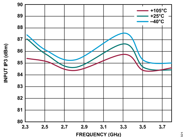
Figure 23. Input IP3 for RF3 vs. Frequency over Various Temperatures
