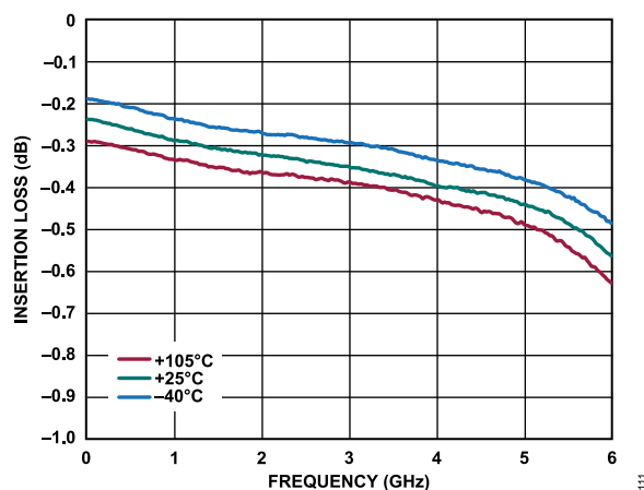
Figure 11. Insertion Loss for RFC to RF1 Selected vs. Frequency over Various Temperatures
