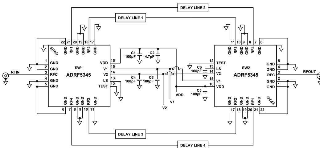
Figure 26. Back to Back Configuration Schematic
