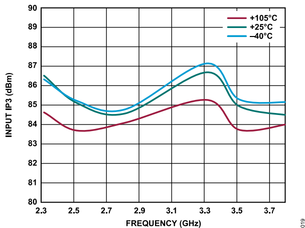
Figure 21. Input IP3 for RF1 vs. Frequency over Various Temperatures
