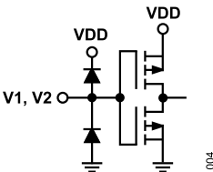
Figure 6. V1 and V2 Control Interface Schematic
