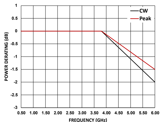
Figure 3. Power Derating vs. Frequency, High Frequency Detail, Tcase = 105C
