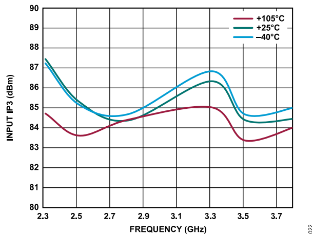
Figure 24. Input IP3 for RF4 vs. Frequency over Various Temperatures
