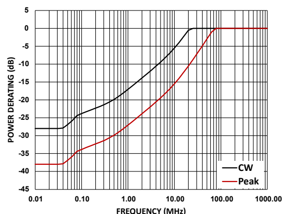
Figure 2. Power Derating vs. Frequency, Low Frequency Detail, Tcase = 105C
