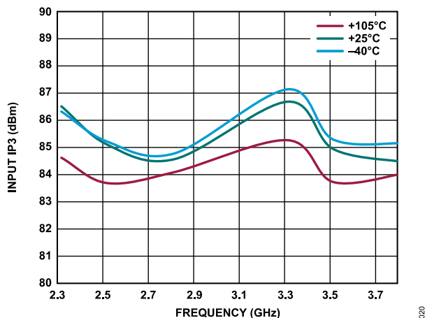
Figure 22. Input IP3 for RF2 vs. Frequency over Various Temperatures
