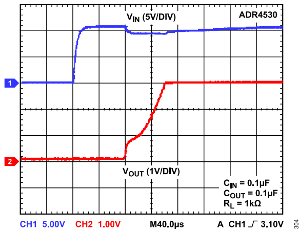
Figure 40. ADR4530 Output Voltage Start-Up Response
