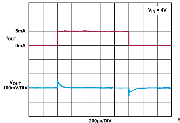
Figure 31. ADR4525 A, B, and C Grades Load Transient Response (Sinking)
