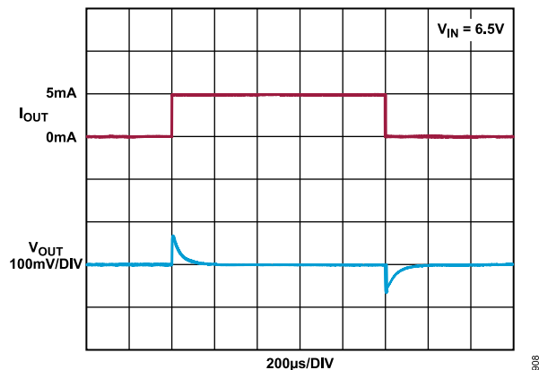
Figure 99. ADR4550 A, B, and C Grades Load Transient Response (Sinking)
