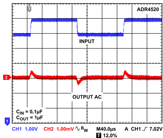
Figure 15. ADR4520 Line Transient Response
