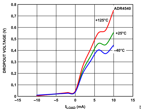
Figure 69. ADR4540 Dropout Voltage vs. Load Current
