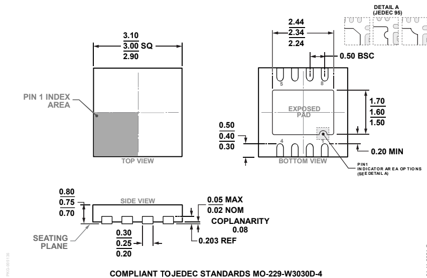
Figure 51. 8-Lead Lead Frame Chip Scale Package [LFCSP] 3 mm × 3 mm Body and 0.75 mm Package Height (CP-8-11) Dimensions shown in millimeters
