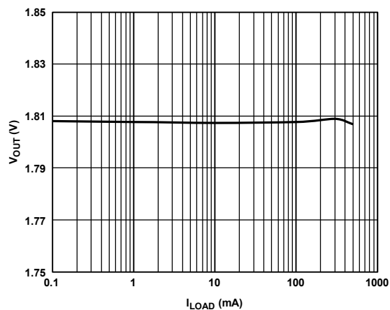
Figure 19. Output Voltage ( V_{OUT} ) vs. Load Current ( I_{LOAD} ), V_{OUT} = 1.8V
