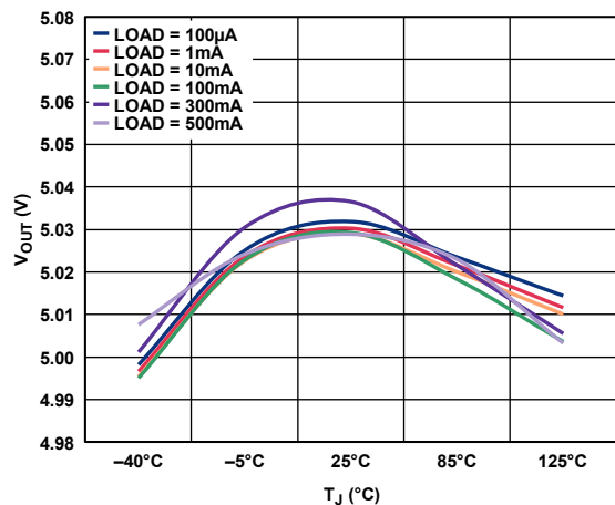
Figure 24. Output Voltage ( V_{OUT} ) vs. Junction Temperature ( T_J ), V_{OUT} = 5V , Adjustable
