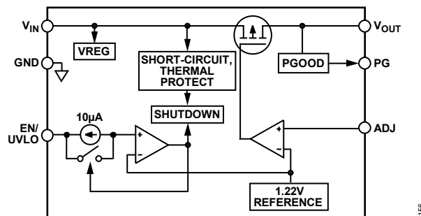
Figure 40. Adjustable Output Voltage Internal Block Diagram
