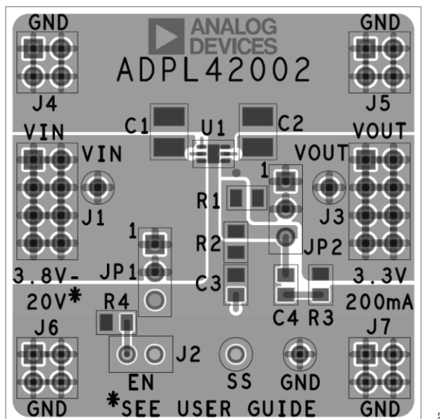
Figure 33. Example LFCSP PCB Layout
