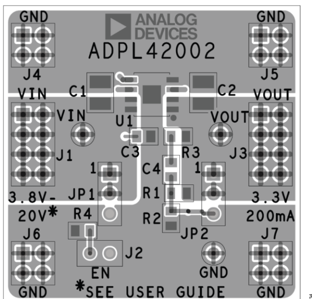
Figure 34. Example SOIC PCB Layout
