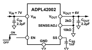
Figure 2. ADPL42002 with 5V Output Adjusted to 6V
