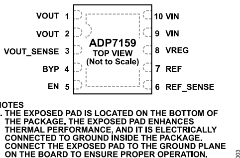
Figure 3. 10-Lead LFCSP Pin Configuration
