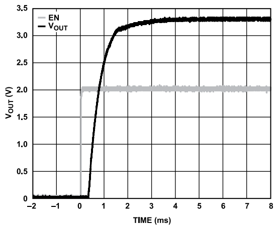
Figure 50. Typical VOUT Response to EN Pin Operation (VEN), VOUT = 3.3 V, VIN = 5 V, CBYP = 1 μF
