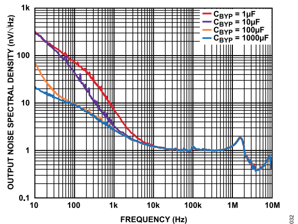
Figure 2. Noise Spectral Density at Different Values of C_{BYP} , V_{OUT} = 3.3 V
