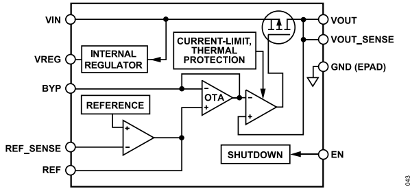
Figure 41. Simplified Internal Block Diagram
