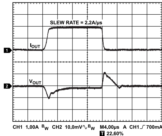
Figure 34. Load Transient Response, I_{LOAD} = 100\text{ mA} to 2\text{ A} , V_{OUT} = 3.3\text{ V} , V_{IN} = 4.0\text{ V} , C_{OUT} = 22\text{ }\mu\text{F} , Channel 1 = I_{OUT} , Channel 2 = V_{OUT}
