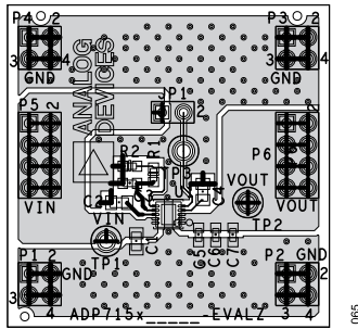
Figure 63. Sample 10-Lead LFCSP PCB Layout
