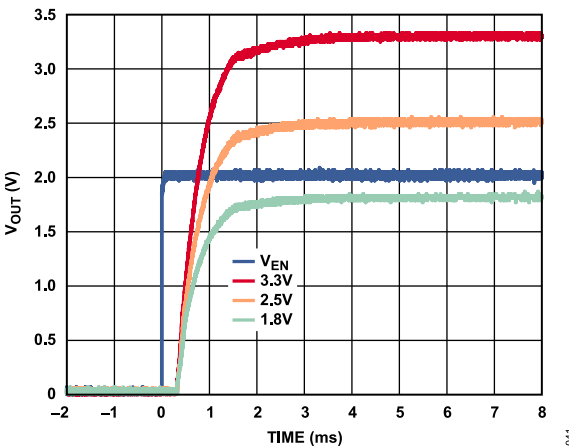
Figure 39. V_{OUT} Start-Up Time After V_{EN} Raising at Various Output Voltages, V_{IN} = 5 \text{ V} , C_{BYP} = 1 \mu\text{F}
