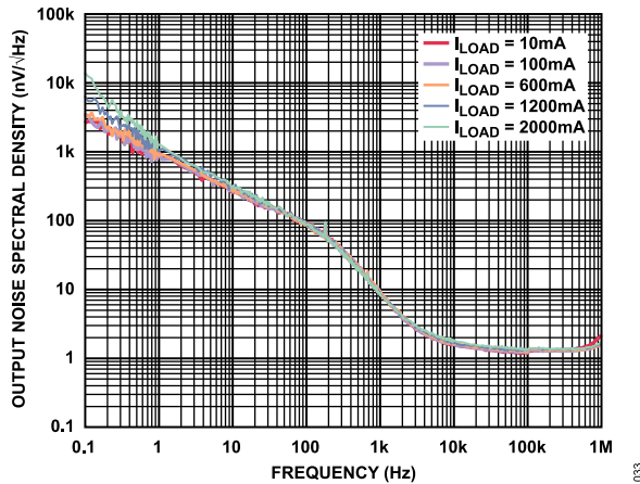
Figure 31. Output Noise Spectral Density at Various Loads, 0.1 Hz to 1 MHz
