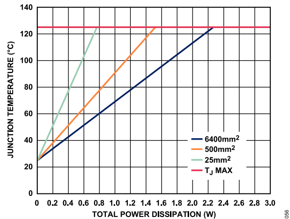
Figure 54. Junction Temperature vs. Total Power Dissipation for the 10-Lead LFCSP, T_A = 25^\circ\text{C}
