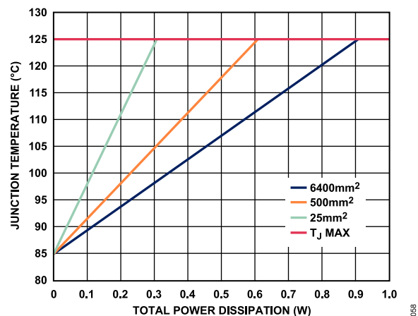
Figure 56. Junction Temperature vs. Total Power Dissipation for the 10-Lead LFCSP, T_A = 85^\circ\text{C}
