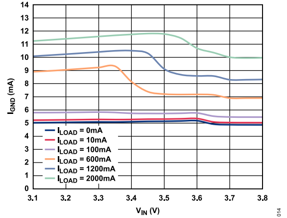
Figure 14. Ground Current ( I_{GND} ) vs. Input Voltage ( V_{IN} ) at Various Loads in Dropout, V_{OUT} = 3.3\text{ V}
