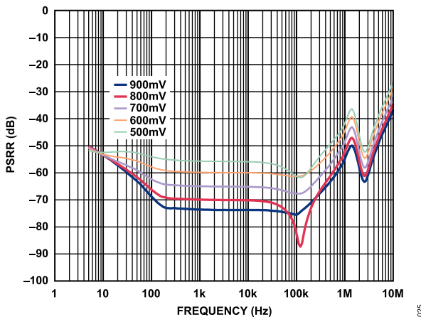
Figure 25. PSRR vs. Frequency at Various Headroom Voltages, V_{OUT} = 1.8\text{ V} , 2 A Load
