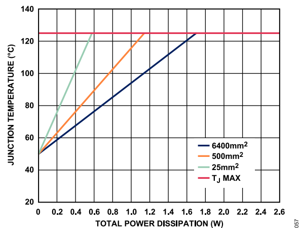
Figure 55. Junction Temperature vs. Total Power Dissipation for the 10-Lead LFCSP, T_A = 50^\circ\text{C}
