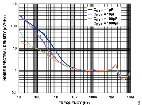
Figure 2. Noise Spectral Density at Various Values of C_{\text{BY}} , V_{\text{OUT}} = 3.3 \text{ V}
