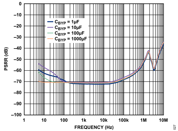
Figure 27. PSRR vs. Frequency at Various C_{BYP} Values, V_{OUT} = 3.3\text{ V} , V_{IN} = 4.0\text{ V} , 2 A Load
