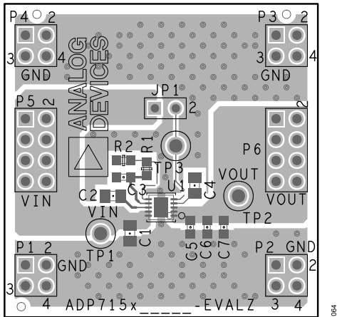
Figure 62. Sample 10-Lead LFCSP PCB Layout
