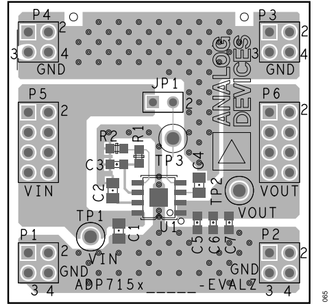
Figure 63. Sample 8-Lead SOIC PCB Layout
