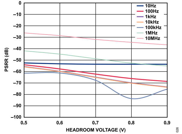
Figure 26. PSRR vs. Headroom Voltage at Various Frequencies, V_{OUT} = 1.8\text{ V} , 2 A Load
