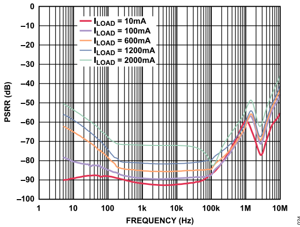
Figure 24. PSRR vs. Frequency at Various Loads, V_{OUT} = 1.8\text{ V} , V_{IN} = 2.6\text{ V}
