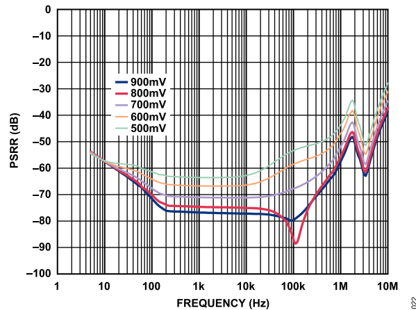
Figure 22. PSRR vs. Frequency at Various Headroom Voltages, V_{OUT} = 3.3\text{ V} , 2\text{ A Load}
