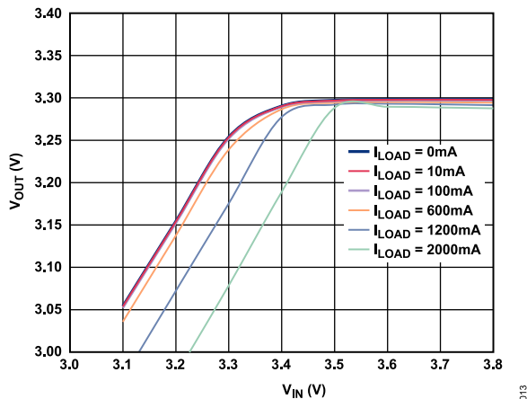
Figure 13. Output Voltage ( V_{OUT} ) vs. Input Voltage ( V_{IN} ) at Various Loads in Dropout, V_{OUT} = 3.3\text{ V}
