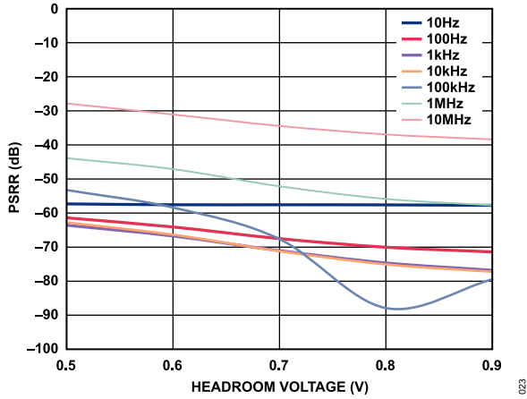
Figure 23. PSRR vs. Headroom Voltage at Various Frequencies, V_{OUT} = 3.3\text{ V} , 2 A Load
