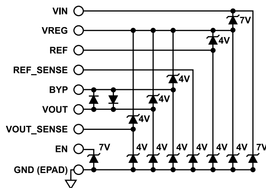
Figure 42. Simplified ESD Protection Block Diagram
