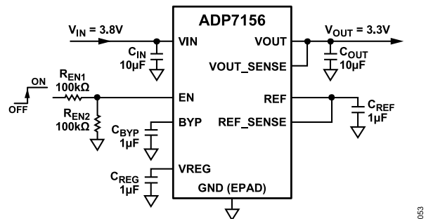
Figure 50. Typical EN Pin Voltage Divider
