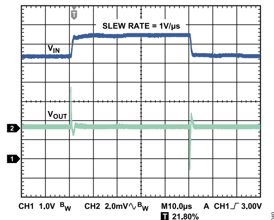
Figure 37. Line Transient Response, 1 \text{ V} Input Step, I_{LOAD} = 1.2 \text{ A} , V_{OUT} = 1.8 \text{ V} , V_{IN} = 2.5 \text{ V} , Channel 1 = V_{IN} , Channel 2 = V_{OUT}
