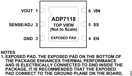
Figure 3. 6-Lead LFCSP Pin Configuration
