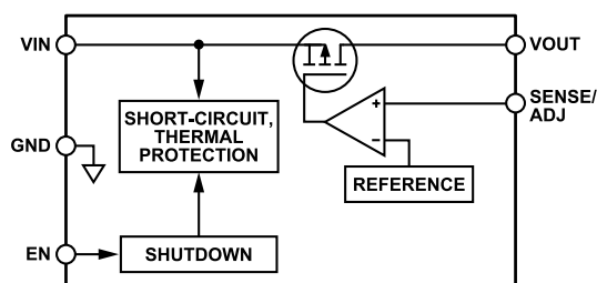
Figure 42. Internal Block Diagram
