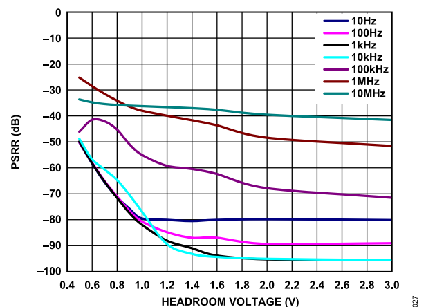
Figure 29. Power Supply Rejection Ratio (PSRR) vs. Headroom Voltage, V_{OUT} = 3.3 V, for Different Frequencies
