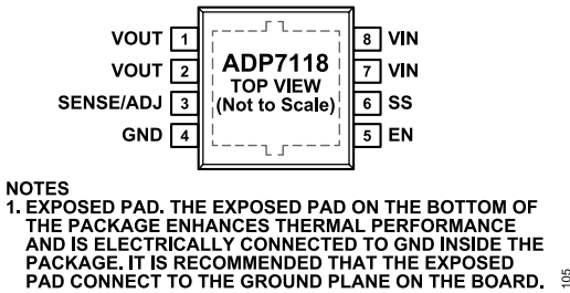
Figure 5. 8-Lead SOIC Pin Configuration
