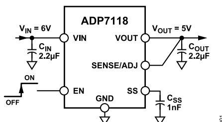
Figure 1. ADP7118 with Fixed Output Voltage, 5 V
