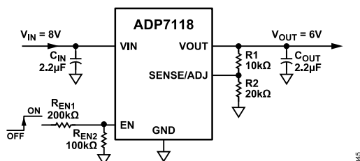
Figure 47. Typical EN Pin Voltage Divider
