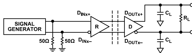
Figure 39. Voltage Definitions
