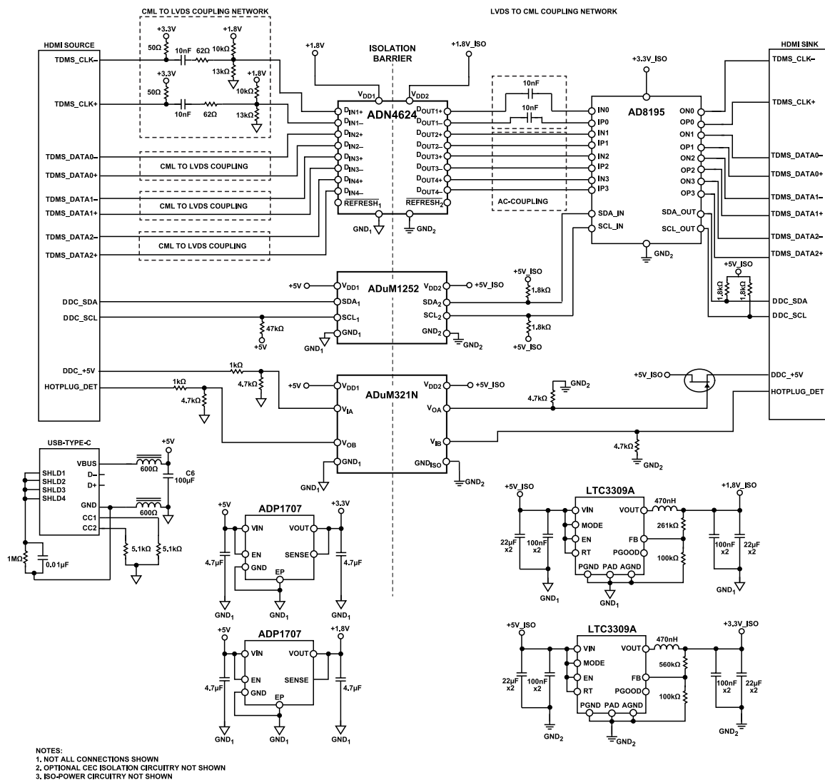
Figure 41. Example Isolated Video Interface (HDMI) Using the ADN4624
