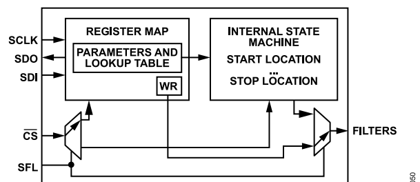
Figure 36. Simplified SPI Diagram
