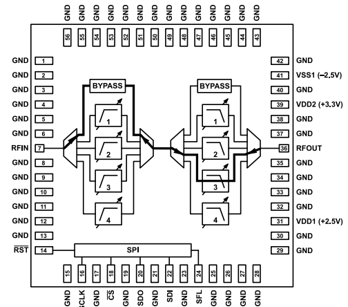
Figure 31. ADMV8818-EP Configured for LPF 3
