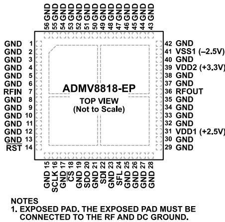
Figure 3. Pin Configuration
