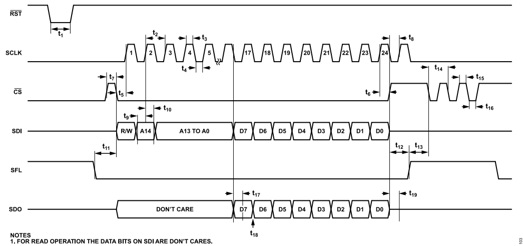
Figure 2. Timing Diagram
