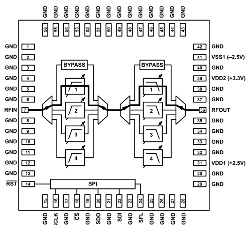
Figure 30. ADMV8818-EP Configured for HPF 1 and LPF 1
