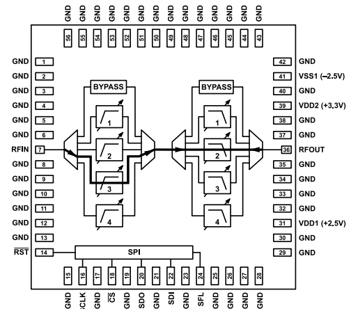
Figure 32. ADMV8818-EP Configured for HPF 3 and LPF 2
