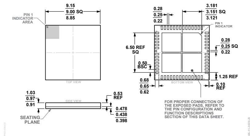
Figure 38. 56-Terminal Land Grid Array [LGA] 9 mm x 9 mm Body and 0.97 mm Package Height (CC-56-3) Dimensions shown in millimeters
