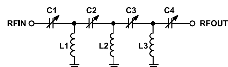
Figure 33. HPF 1 Simplified Schematic
