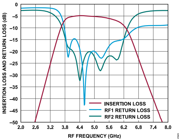
Figure 48. Insertion Loss and Return Loss vs. RF Frequency at HPF and LPF, State 0
