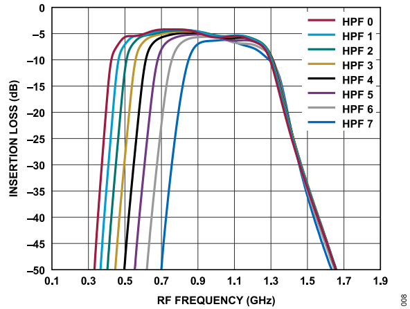
Figure 8. Insertion Loss vs. RF Frequency at LPF, State 7 and Swept HPF State
