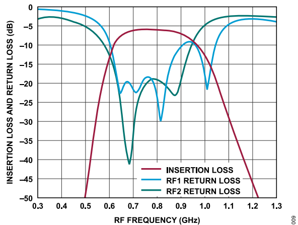
Figure 9. Insertion Loss and Return Loss vs. RF Frequency at HPF and LPF, State 4
