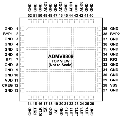
Figure 3. Pin Configuration
