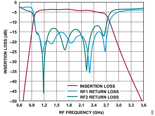
Figure 27. Insertion Loss and Return Loss vs. RF Frequency at HPF, State 0 and LPF, State 7
