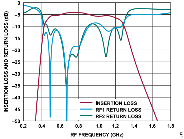
Figure 13. Insertion Loss and Return Loss vs. RF Frequency at HPF, State 0 and LPF, State 7
