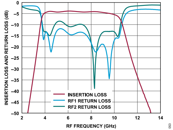
Figure 55. Insertion Loss and Return Loss vs. RF Frequency at HPF, State 0 and LPF, State 7
