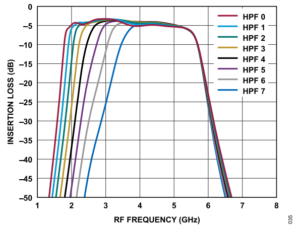
Figure 36. Insertion Loss vs. RF Frequency at LPF, State 7 and Swept HPF State
