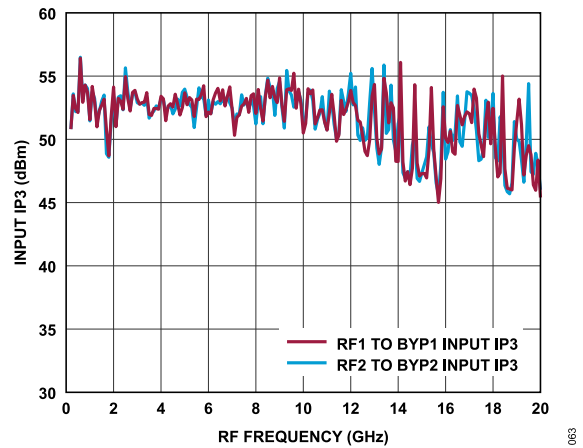
Figure 63. Input IP3 vs. RF Frequency
