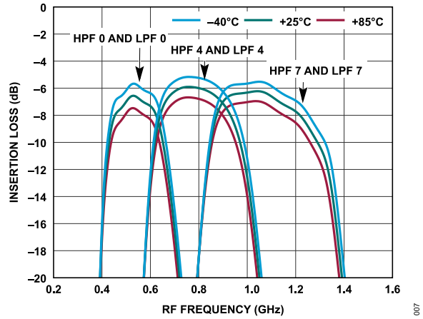
Figure 7. Insertion Loss vs. RF Frequency at HPF and LPF, State 0, State 4, and State 7 in Various Temperatures
