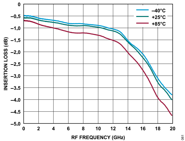
Figure 61. Insertion Loss vs. RF Frequency in Various Temperatures
