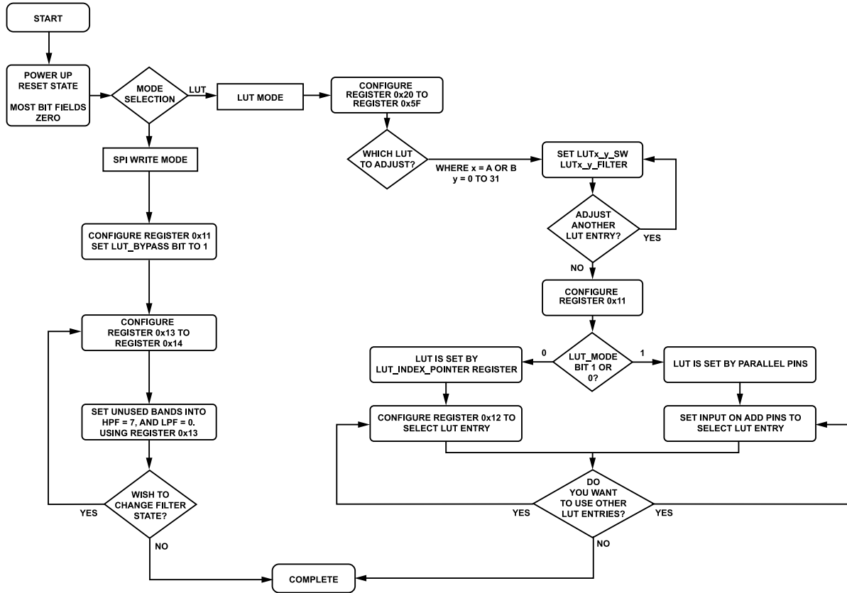
Figure 65. Programming Flow Chart
