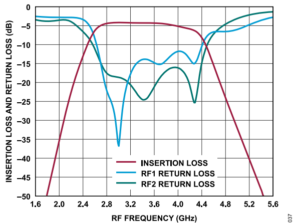
Figure 37. Insertion Loss and Return Loss vs. RF Frequency at HPF and LPF, State 4
