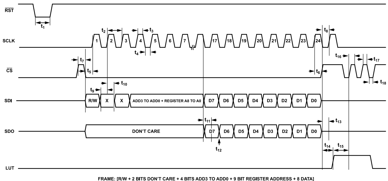
Figure 2. Timing Diagram
