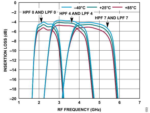
Figure 35. Insertion Loss vs. RF Frequency at HPF and LPF, State 0, State 4, and State 7 in Various Temperatures
