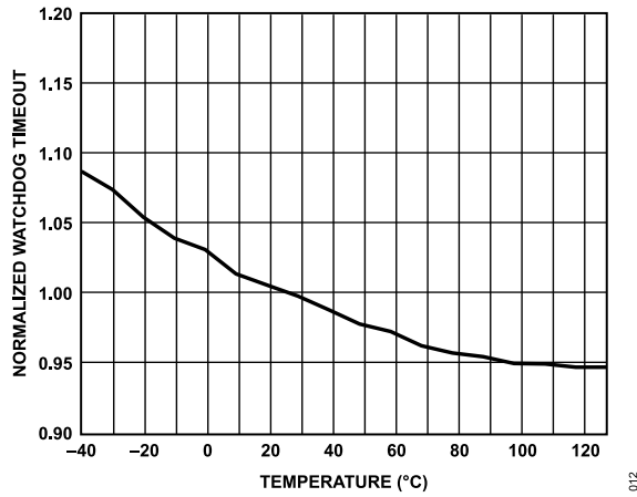
Figure 12. Normalized Watchdog Timeout vs. Temperature
