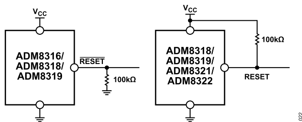
Figure 22. Ensuring Reset Valid to V_{CC} = 0 V
