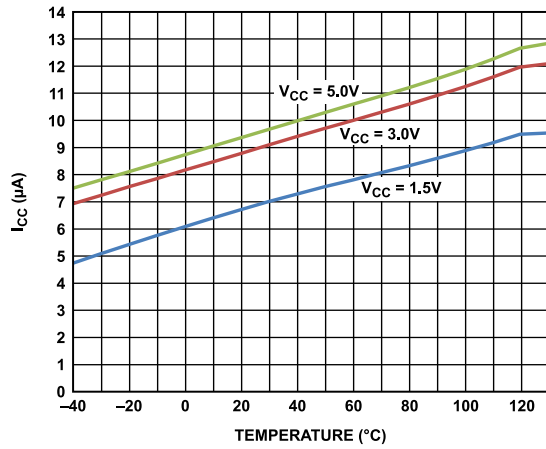
Figure 6. Supply Current ( I_{CC} ) vs. Temperature
