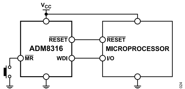
Figure 24. Typical Application Circuit
