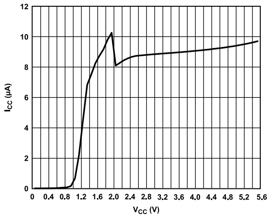
Figure 7. Supply Current ( I_{CC} ) vs. Supply Voltage ( V_{CC} )
