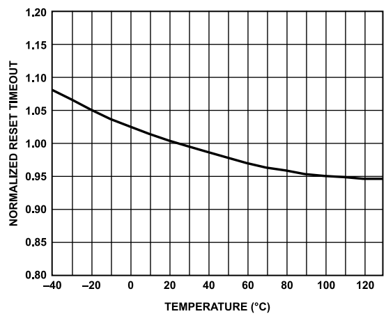
Figure 11. Normalized Reset Timeout vs. Temperature
