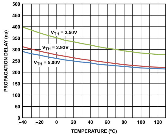
Figure 10. Manual Reset to Reset Propagation Delay vs. Temperature
