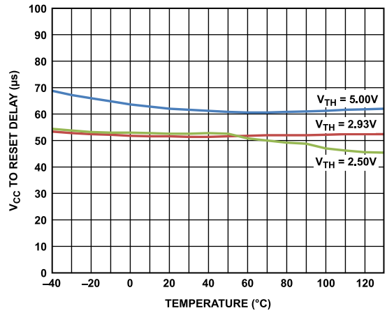
Figure 9. V_{CC} to Reset Delay vs. Temperature
