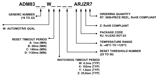
Figure 25. Ordering Code Structure
